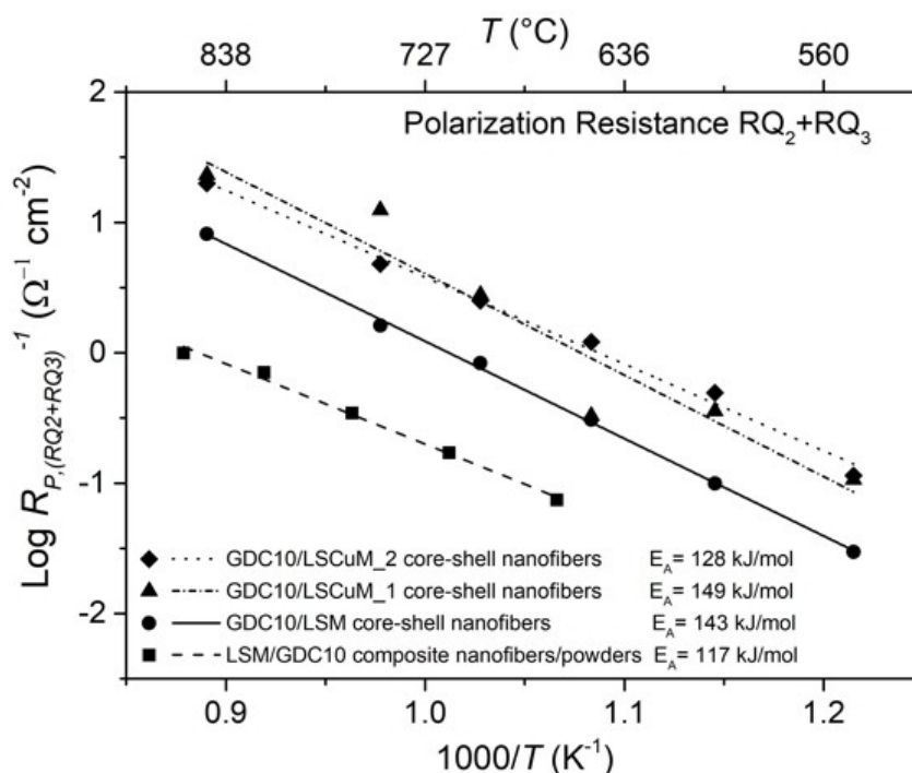
Figure 11. Arrhenius plot of R_{P_i/(R_{Q2}+R_{Q3})}^{-1} of GDC10/LSM, GDC10/LSCuM_1 and GDC10/LSCuM_2 core-shell nanofiber cathodes. These are compared with the LSM/GDC10 composite nanofibers/powders electrode (LSM nanofibers mixed with GDC10 powders). [32]
