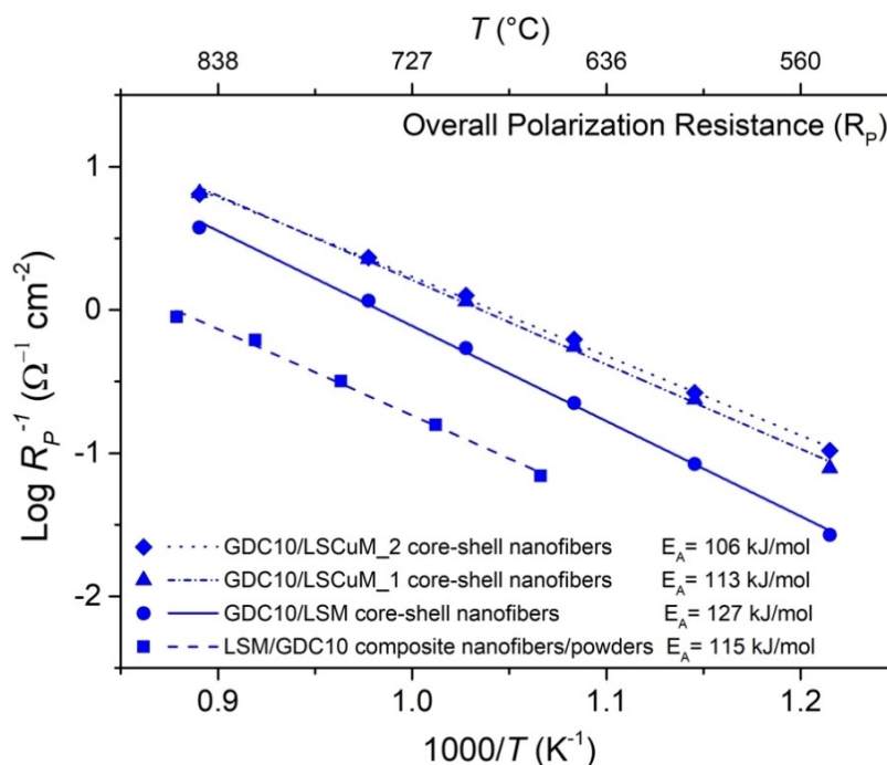
Figure 9. Arrhenius plot of R_p^{-1} for GDC10/LSM, GDC10/LSCuM_1, and GDC10/LSCuM_2 core-shell nanofiber cathodes. These are compared with the LSM/GDC10 composite nanofiber/powder electrode (LSM nanofibers mixed with GDC10 powders). [32]
