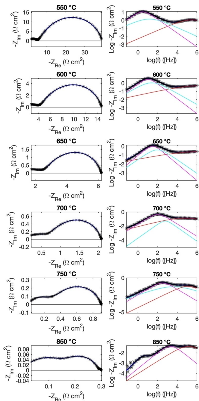
Figure 5. Nyquist (left) and Bode (right) plots of the EIS measurements on the GDC10/LSM core-shell nanofiber electrode at temperatures from 550 °C to 850 °C, in air atmosphere: *experimental data; — fitting through the Rs-RQ1-RQ2-RQ3 equivalent circuit model; — RQ1 contribution; — RQ2 contribution; — RQ3 contribution (vanishing at 850 °C).
