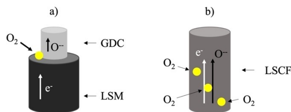
Figure 6. The charge transfer process in composite (a) and MIEC (b) cathodes. The • represents the reaction active site.
