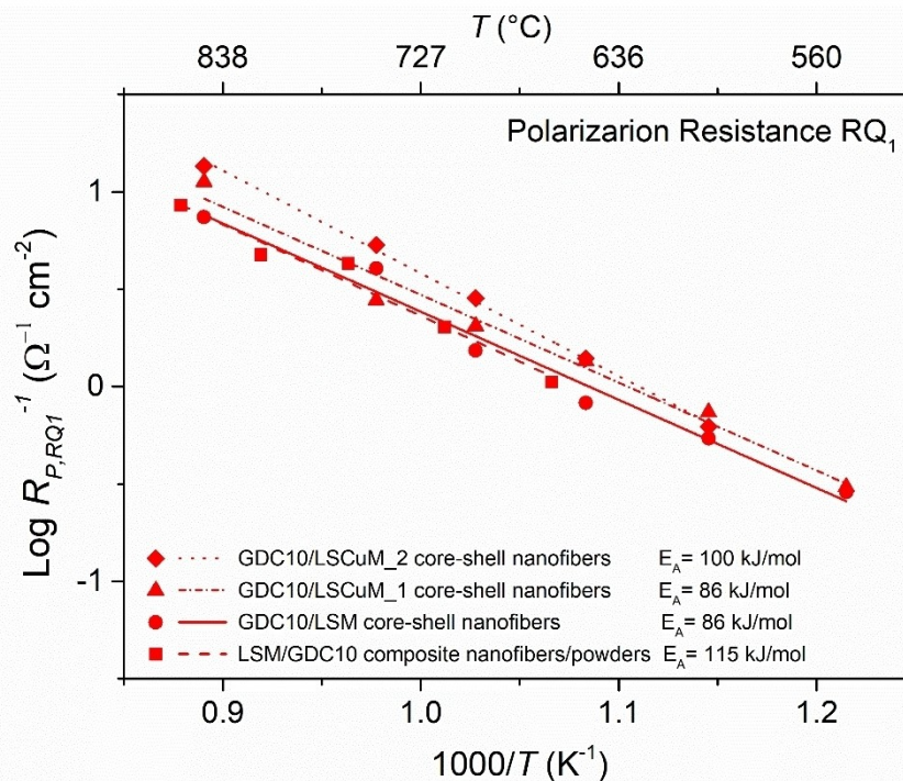
Figure 10. Arrhenius plot of R_{p,RQ1}^{-1} of GDC10/LSM, GDC10/LSCuM_1 and GDC10/LSCuM_2 core-shell nanofiber cathodes. These are compared with the LSM/GDC10 composite nanofiber/powder electrode (LSM nanofibers mixed with GDC10 powders). [32]
