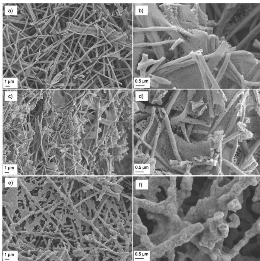
Figure 2. Core-shell nanofibers after the EIS measurements. (a–b) GDC10/LSM, (c–d) GDC10/LSCuM_1 and (e–f) GDC10/LSCuM_2.
