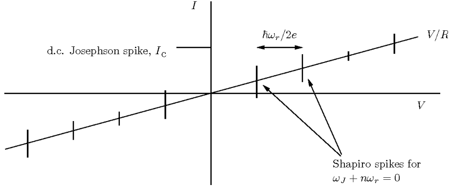
Figure 2.4: DC current of a Josephson junction driven by an AC voltage, with the well visible Shapiro spikes of width \hbar\omega_r/2e . Figure adapted from [135].
