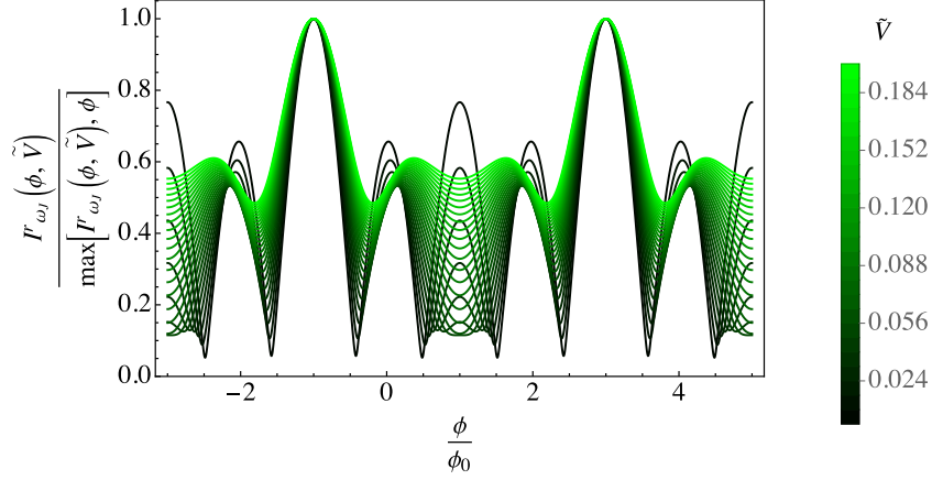
Figure 3.8: I_{\omega_J}^r , normalized with respect to its maximum, for \tilde{L} = 20 , k_F L = 6\pi , \tilde{f}_T = 0.4 , f_C = 0.3 , \tilde{f} = 0.3 and \tilde{T} = 0.1 . The plot is represented as a function of \phi (in units of \phi_0 ) and for \tilde{V} varying between 0.008 and 0.2 (see the green bar legend aside). Figure adapted from [188].
