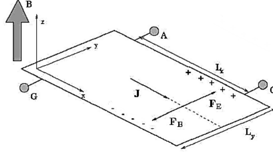
Figure 1.1: The Hall bar. The magnetic field B is directed along the z direction, and an in-plane electric field \mathbf{E} pushes electrons to move creating a current density \mathbf{J} . Due to the magnetic contribution to the Lorentz force, denoted by \mathbf{F}_B electrons accumulate on the upper edge of the bar. Due to the imbalance of charge between the two edges of the bar, an electric component of the Lorentz force \mathbf{F}_E arises. When they compensate, the only surviving component of the current density is along the x direction.
