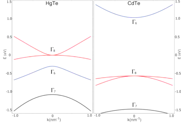
Figure 1.11: Bulk energy bands of HgTe and CdTe near the \Gamma -point. The \Gamma_8 band is indicated in red and the \Gamma_6 band is indicated in blue. Figure from [21], reprinted with permission from AAAS.
