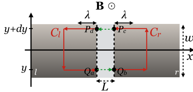
Figure 2.6: Sketch of the junction under consideration, having width w and barrier's thickness L . The two superconductors are labeled by r, l and assumed to have the same London penetration depth \lambda . The London penetration depth represents the characteristic decay length over which an applied field decays exponentially inside a superconductor.
