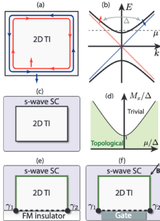
Figure 1.29: (a) Schematic of the system, consisting in the two counter-propagating, helical edge states of a Quantum Spin Hall Insulator in a ring geometry. (b) The bare edge states' dispersion (red and blue lines) and the modified spectrum in the presence of a Zeeman term (black solid lines). (c) The system is proximitized by a s -wave superconductor, which pushes the edge into a topological superconducting phase such as the weak-pairing phase in Kitaev model. (d) Phase diagram of the system, elucidating the trivial and topological regimes as a function of M_x and \mu . (e)-(f) Domain walls between topological (green lines) and trivial regions (dashed lines) localize Majorana zero-modes (denoted by \gamma_{1,2} ). This can be done either with a ferromagnetic insulator (e) or with a Zeeman field with a proper tuning of \mu by gating (f). Figure adapted with permission of IOP Publishing, Ltd, from [3]; permission conveyed through Copyright Clearance Center, Inc.
