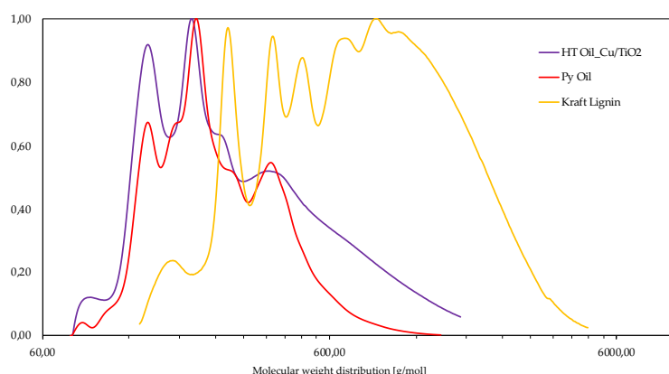
Figure 56: GPC profiles of initial kraft lignin (yellow), pyrolysis oil (red), and hydrotreated oil (purple).
