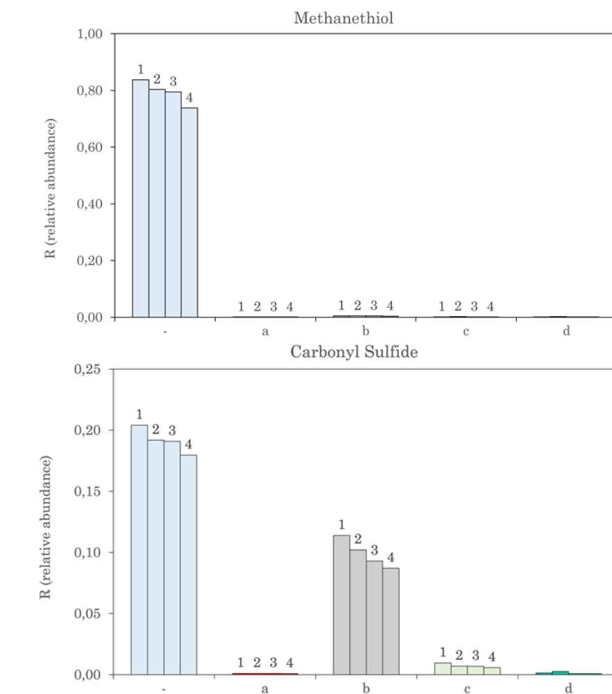
Figure 32: GC-MS for quantitative analysis of Hydrogen sulfide, methanethiol and carbonyl sulfide present in the pyrolytic gas. Each histogram represents a different injection in GC-MS (four each test). Data reported are related to average values obtained without adsorption bed and to values obtained after the adsorption on four different activated carbons (a-Carbosorb MA 1.5, b-Carbosorb 360 C3, c-Carbosorb 53, d-Carbosorb 73).
