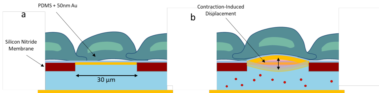
Figure 4.1 Scheme of single cell micro interferometer. a) It shows a static scheme of the single cell micro interferometer; each PDMS window is 30μm of diameter and it is 1-2 μm thick. b) Scheme of the contraction-induced displacement of the PDMS layer.
