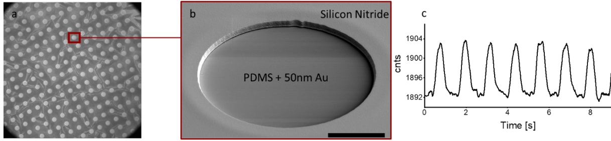
Figure 4.2 a) Optical image of the single cell resolution device. b) SEM image of the PDMS window surrounded by the silicon nitride substrate. Each window has a diameter of 30 \mu\text{m} . c) Example of contraction signal coming from a single cell micro-interferometer.
