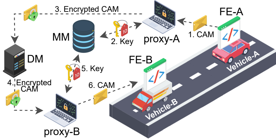
Figure 2.3: Data flow in the cooperative lane change service
