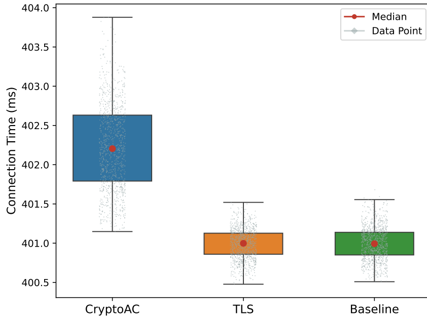
Figure 4.7: Overhead of the communication setup for CryptoAC, TLS, and the baseline configurations
