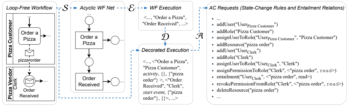
Figure 3.4: Application of ACE on (a portion of) The Pizza Collaboration BPMN workflow
