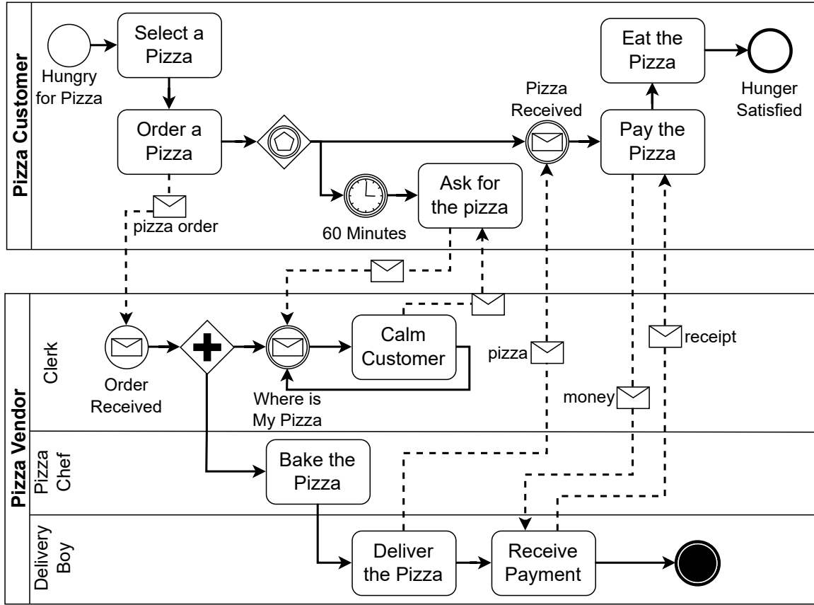
Figure 3.1: BPMN workflow - The Pizza Collaboration
