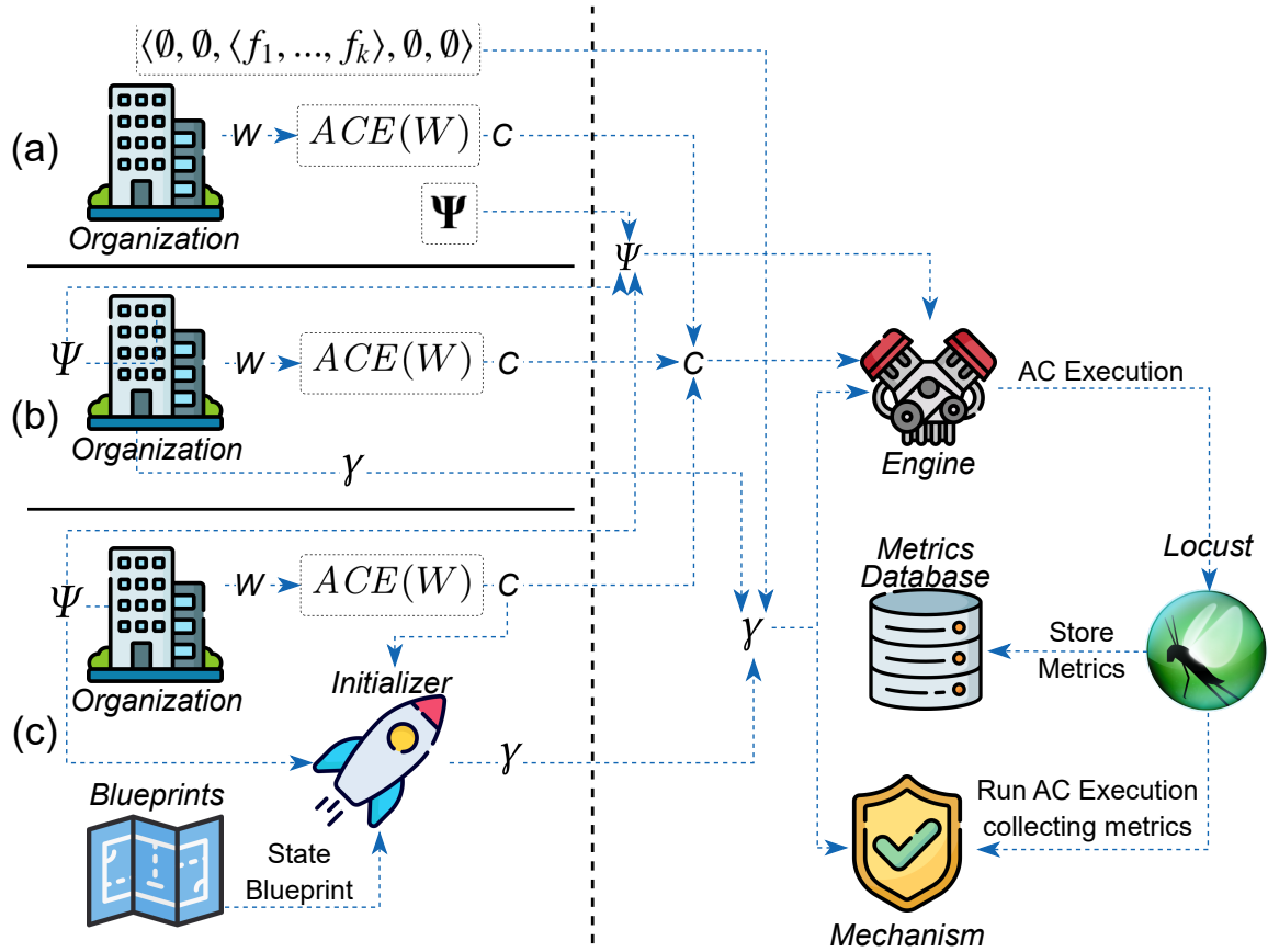
Figure 3.5: Representation of ACME in the context of our methodology for (a) basic, (b) highly customized, and (c) partially customized RBAC System
