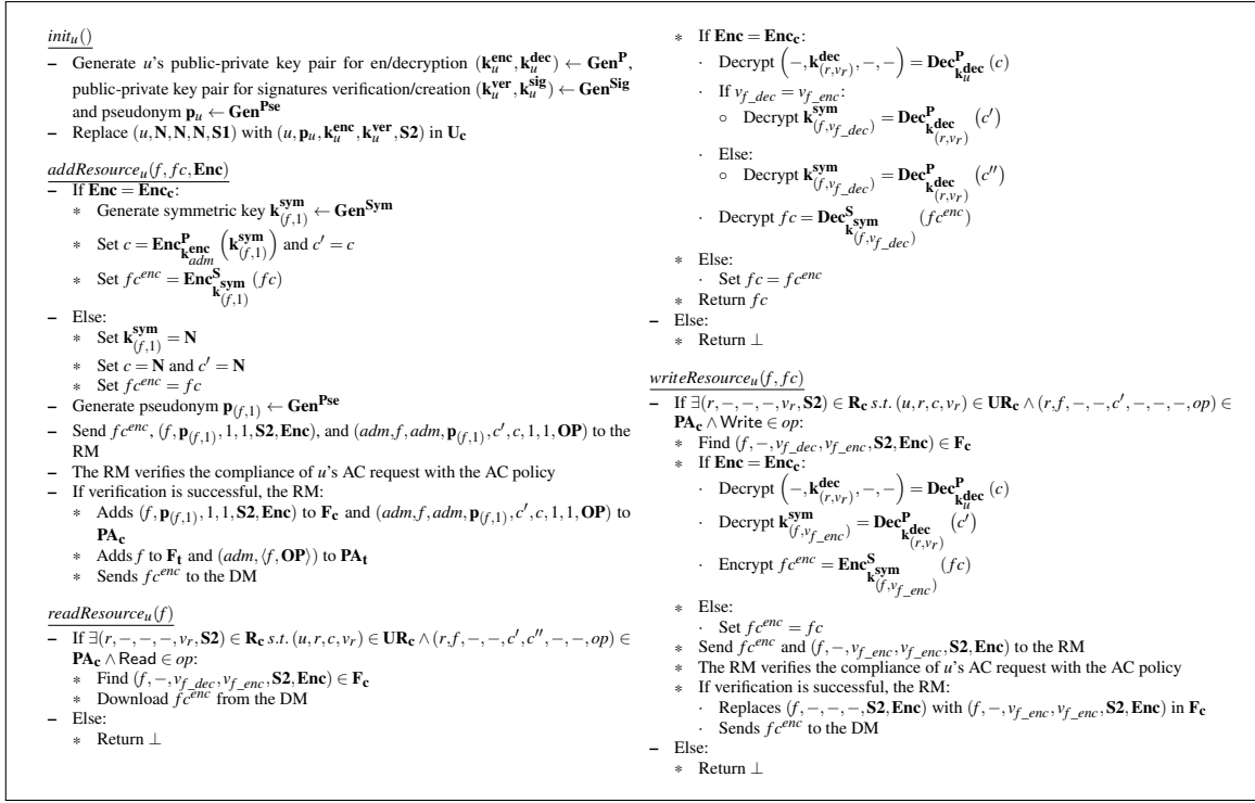
Figure 4.2: Pseudocode for the user operations of the CAC scheme for RBAC
