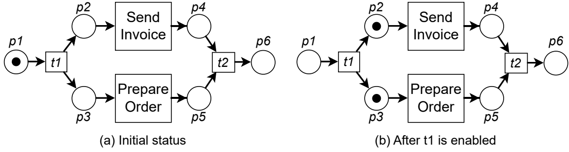
Figure 3.2: Sample WF net
