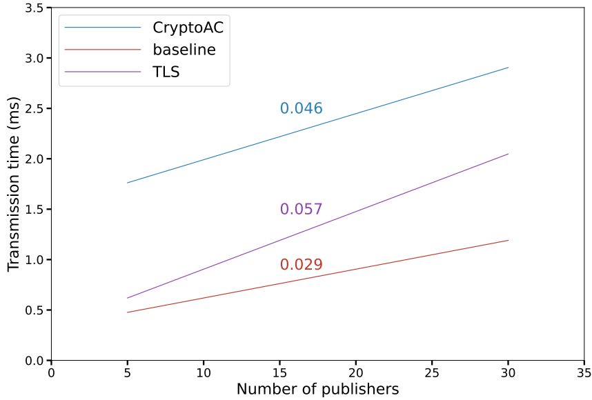
Figure 4.8: Overhead of the communication for CryptoAC, TLS, and the baseline configurations
