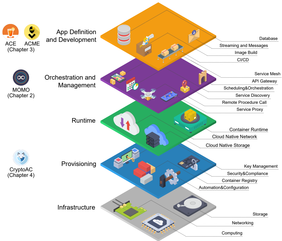
Figure 1.1: The cloud native stack of CNCF
