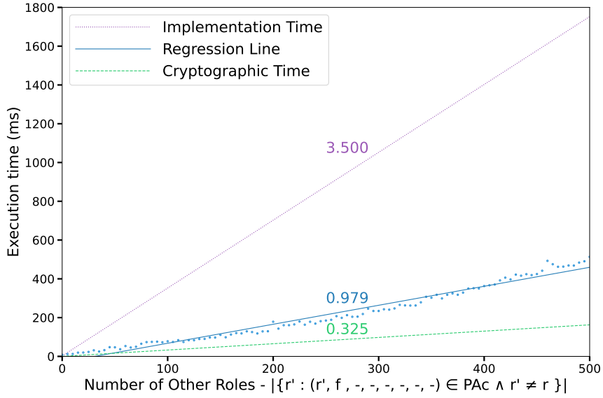
Figure 4.10: Performance of \text{revokePermissionFromRole}_{adm}(r, \langle f, op \rangle)
