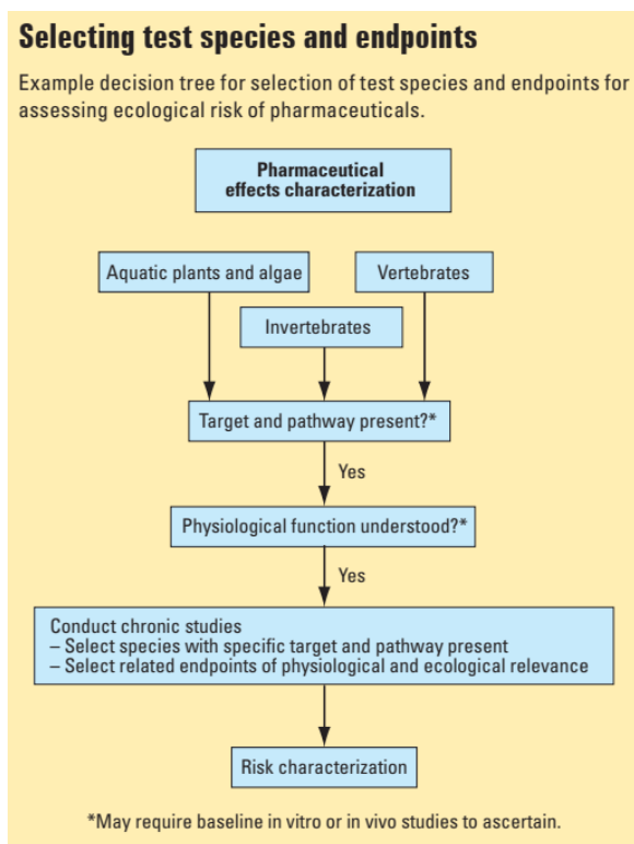
Figure 3.1. Schematic representation of characterisation of risk assessment.
