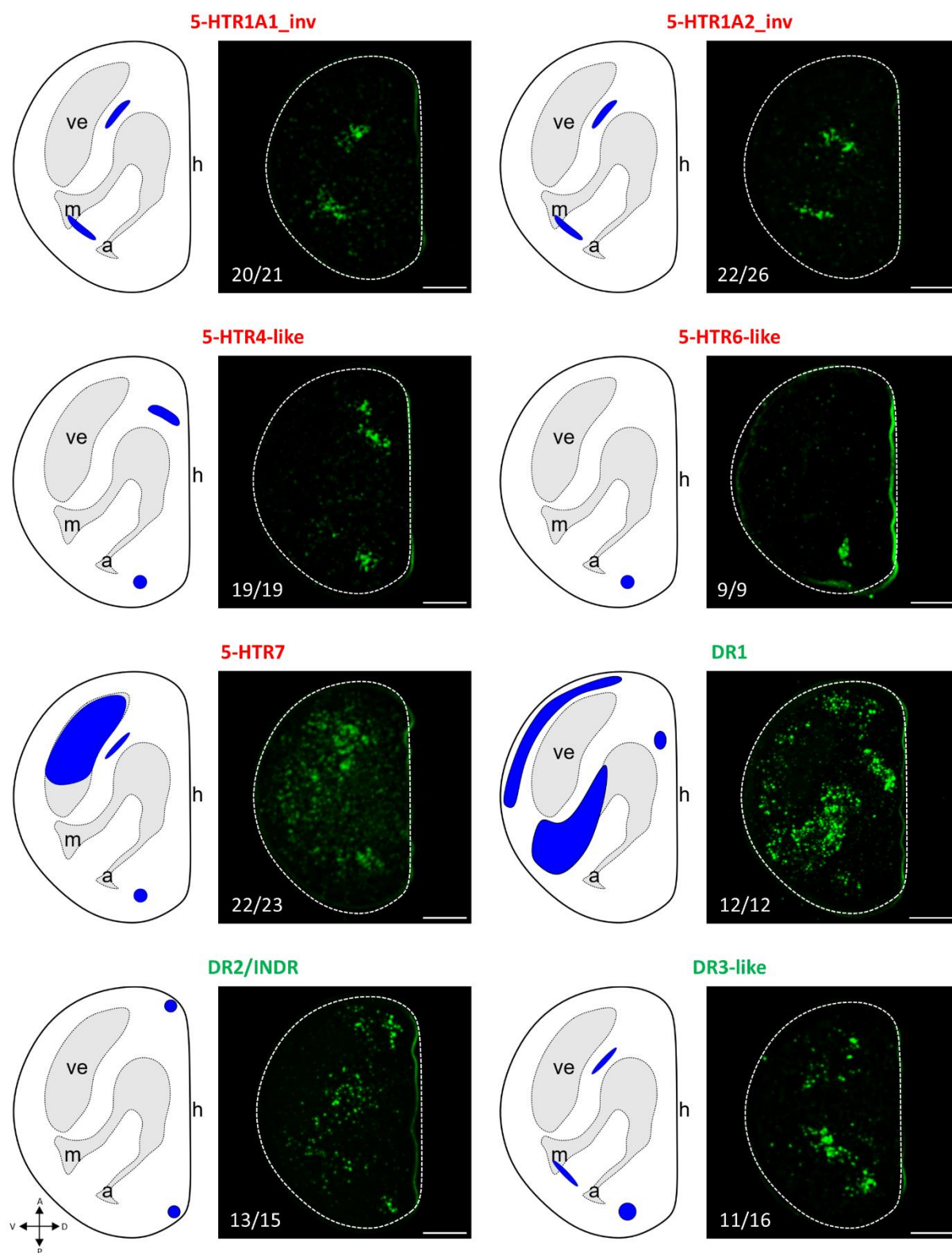
Supplementary Figure 6.16. Representative images of single HCR of the 5-HTRs (red title) and DRs (green title) analysed. For each confocal images a scheme representing the signal in reported on the left. The number of larvae presenting the signal drawn in the scheme is reported on the left corner of confocal images. Scale bar: 20 \mu m.
