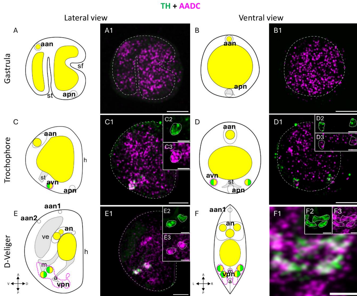
Supplementary Figure 6.18. Spatiotemporal localisation of AADC and TH during M. galloprovincialis embryo-larval development. Double HCR with TH (B2 amplifier) and AADC (B1 amplifier) was used. TH signal is represented in green in both schemes and HCR images; AADC signal is represented in yellow and in magenta in schemes and HCR images, respectively. 7B2 area is represented in schemes by dotted lines and by neuronal clusters names. The white colour in confocal images is the result of green and magenta colocalisation.
