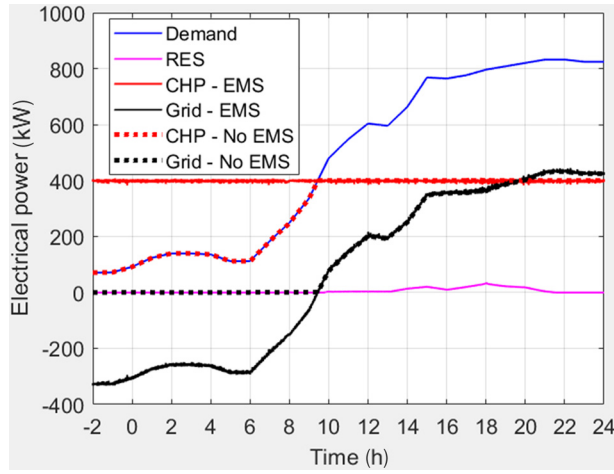
Fig. 10 Electrical power comparison (EMS versus no EMS cases) for the €5/MWh syngas cost
