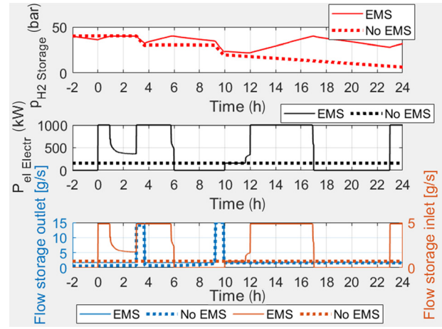
Fig. 12 Comparison (EMS versus no EMS cases) for the hydrogen generation, storage, and utilization (€5/MWh syngas cost)
