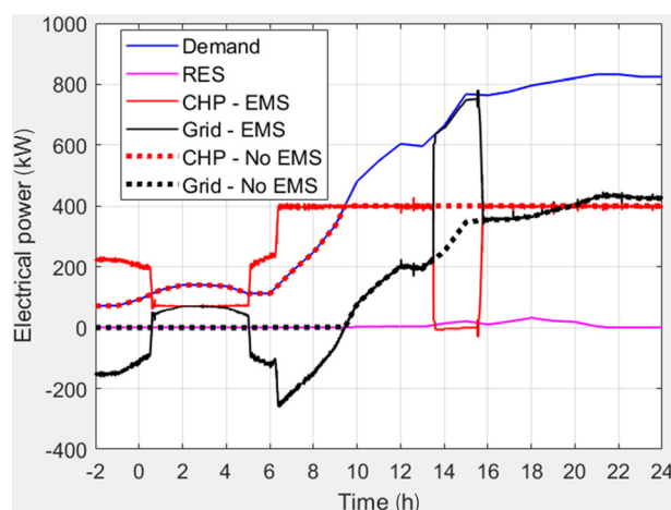
Fig. 7 Electrical power comparison (EMS versus no EMS cases) for the €80/MWh syngas cost
