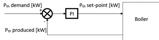
Fig. 6 PI tool for the boiler set-point calculation in the no EMS cases
