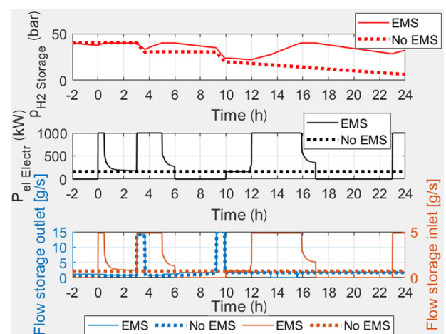
Fig. 9 Comparison (EMS versus no EMS cases) for the hydrogen generation, storage, and utilization (€80/MWh syngas cost)
