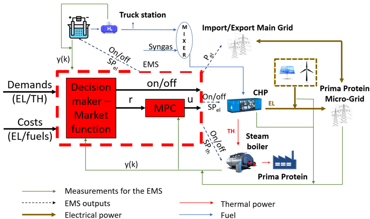
Fig. 1 Plant layout and EMS integration
