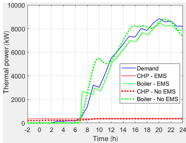
Fig. 11 Thermal power comparison (EMS versus no EMS cases) for the €5/MWh syngas cost
