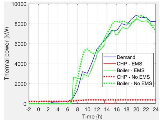
Fig. 8 Thermal power comparison (EMS versus no EMS cases) for the €80/MWh syngas cost
