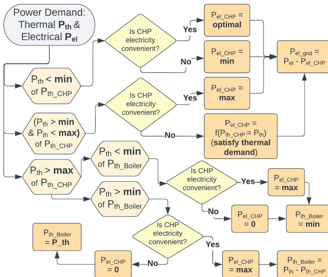
Fig. 2 Flowchart of the EMS logic
