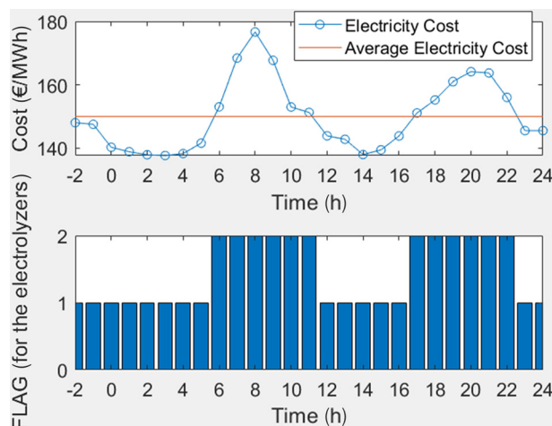
Fig. 3 Electricity costs considered in this article and flags for the management of the electrolyzers
