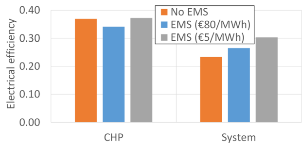
Fig. 14 Comparison of system electrical efficiency for the cases discussed in this paper (full 26-h duration)
