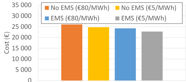
Fig. 13 Comparison of global variable costs for the cases discussed in this paper (full 26-h duration)
