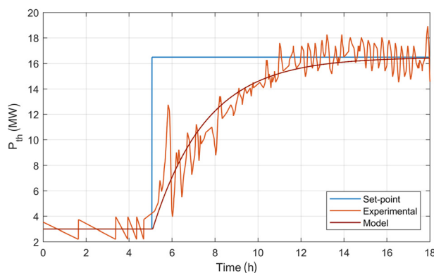
Fig. 5 Boiler model validation
