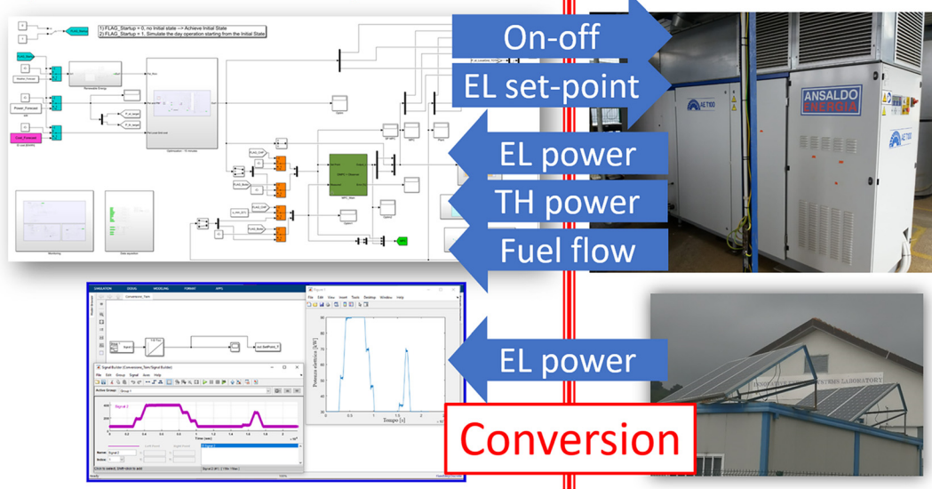
Fig. 4 Hardware/software communication for the cyber-physical approach
