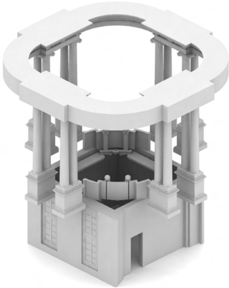
Fig. 5 - Axonometric view of the true space with the projective virtual space (case 2 Fig. 3). (modeling by C. Marino, rendering by G.B. Gheresi).
