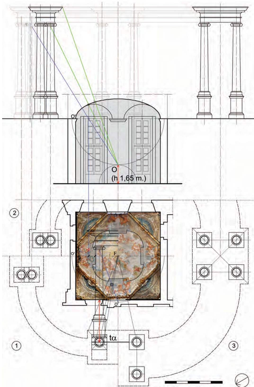
Fig. 3 - Plan and section: the perspective restitution and the hypothetical reconstruction (C. Cândito): 1 - with the ortophoto; 2 - with the vault intersection (see Fig. 5); 3 - Ideal Architecture (see Fig. 6).
