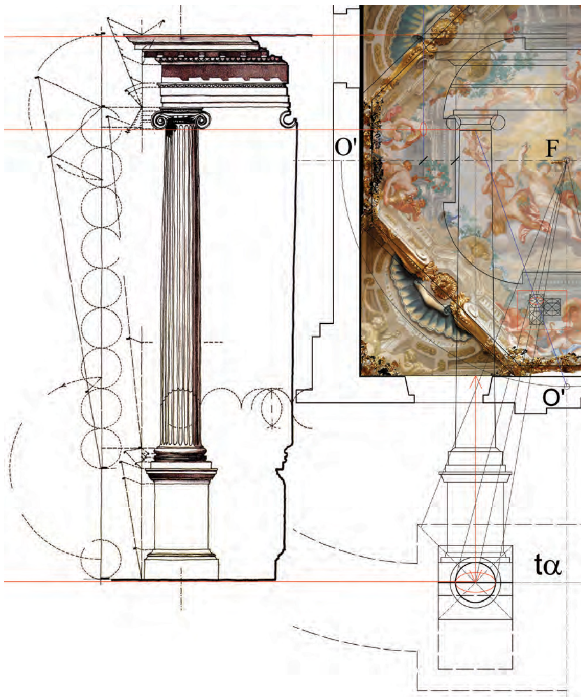
Fig. 4 - On the left: the Ionic order by Andrea Palladio (Migliari R. 1991). On the right: the scale of the Autumn Room order. Using the distance from the hypothetical floor to the necking, one can observe that the imoscape is proportioned with the perspective restitution. (C. Cândiato).
