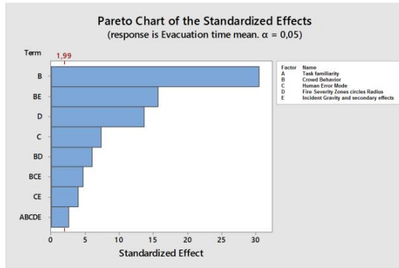
Figure 12. Pareto Chart Analysis for the Evacuation Time
