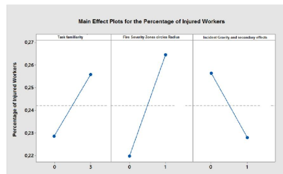
Figure 11. Main Effect Plots for the Percentage of injured workers
