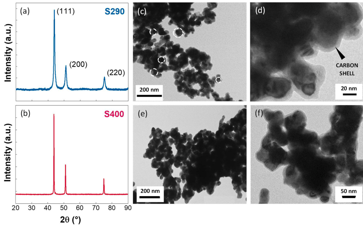
Fig. 2. (a, b) XRD patterns of samples (a) S290 and (b) S400. (c – f) TEM images at different magnifications of samples (c, d) S290 and (e, f) S400.
