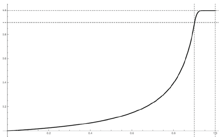
Fig. 2 Numerical plot of the function f_\varepsilon defined in (1.8), obtained by choosing the prototype function f_{(q)} (with q = 1 ) as in Remark 1.3 and the exponential junction \psi_\varepsilon as in Remark 1.4
