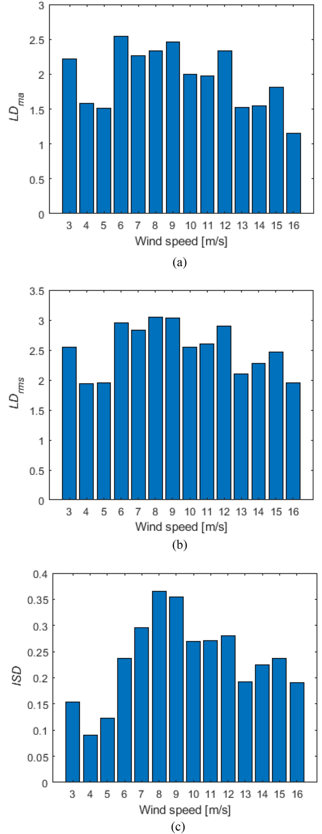
Fig. 4. Performance of predicting the spectral averages of noise measured at turbine A5 by using the spectral averages at turbine A1. (a) Mean absolute log-spectral distance; (b) root mean square log-spectral distance; (c) Itakura-Saito divergence.
