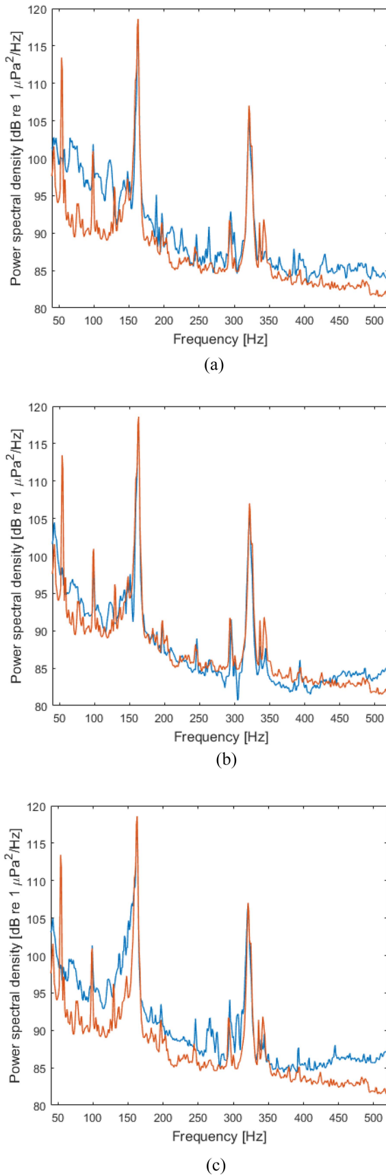
Fig. 12. Prediction of the spectral average at 13 m/s for turbine A5 (brown line) in case study C3. Example of result (blue line) obtained by (a) AAI, (b) PCA and GPR, and (c) NMF and GPR.
