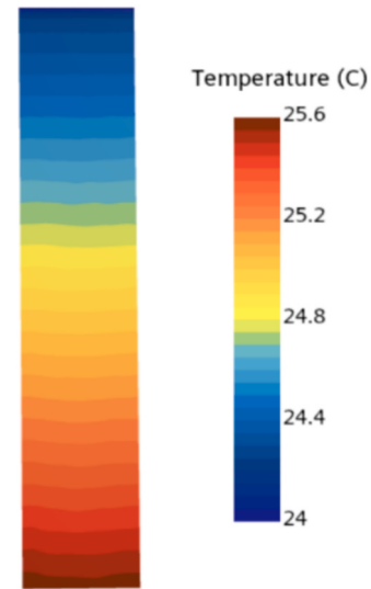
Fig. 6. Steady-state temperature distribution along the plate.
