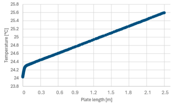
Fig. 6. Steady-state temperature distribution along the plate.
