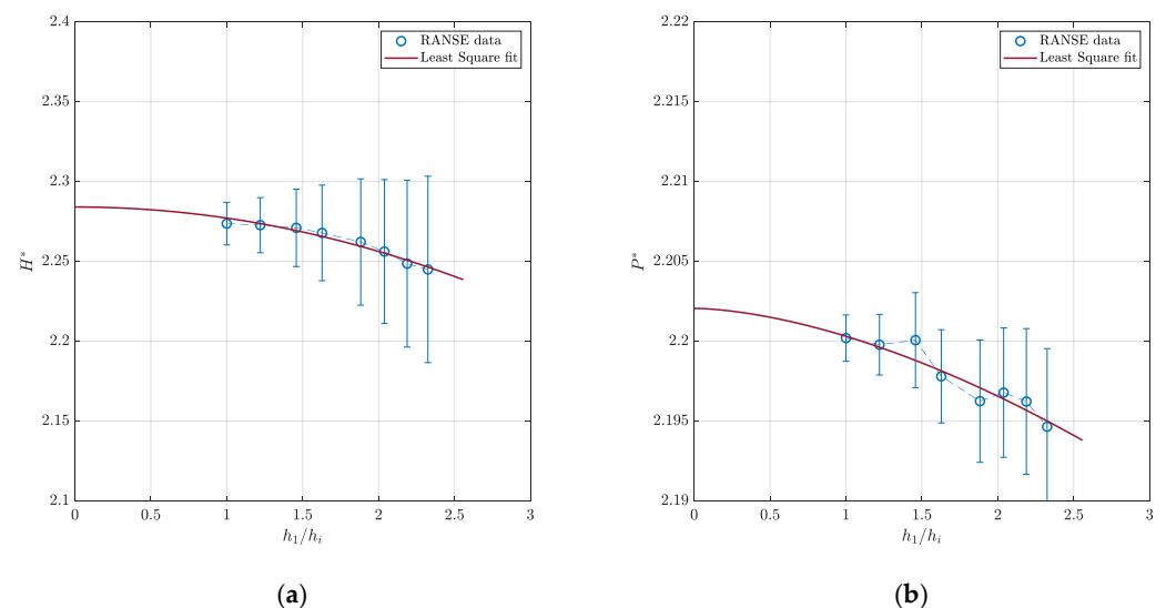
Figure 8. Grid sensitivity and associated numerical uncertainties: head (a) and power (b) coefficients under cavitating conditions ( Q^* = 0.85 , \sigma_N = 5 ).
