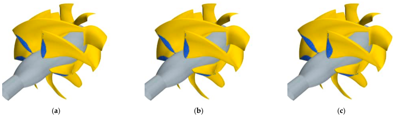
Figure 10. Predicted cavity bubble for different simulation time steps: 2 deg. (a), 0.5 deg. (b), and 0.25 deg. (c) ( Q^* = 0.85 , \sigma_N = 5 ).
