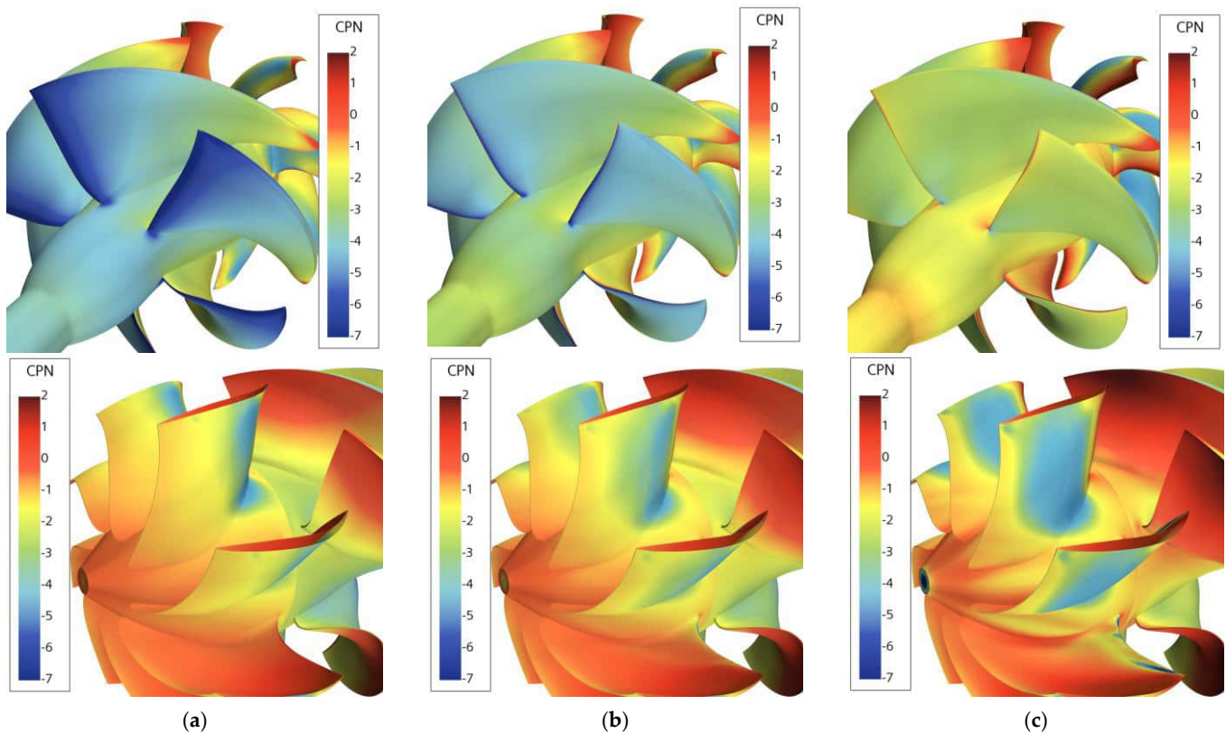
Figure 12. Pressure coefficient ( C_{pN} ) distributions over rotor and stator blades of the reference waterjet. Q^* = 0.75 (a), Q^* = 0.85 (b), and Q^* = 0.95 (c).
