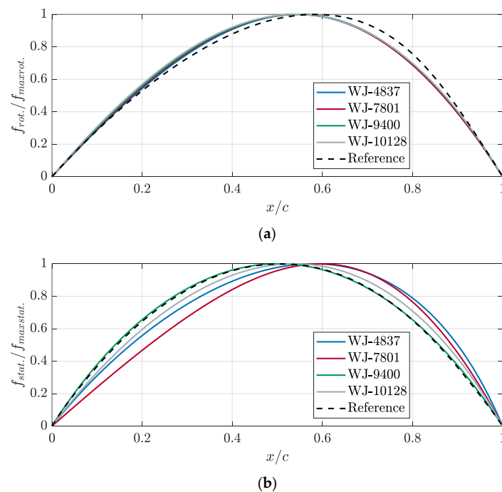
Figure 23. Non-dimensional camber line (with respect to the maximum sectional value, f_{max} ) of the sectional hydrofoils of the rotor (a) and stator (b).
