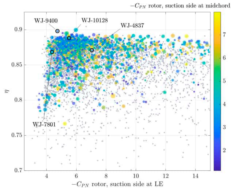
Figure 16. Results of the optimization process. Feasible configurations (efficiency versus risk of cavitation on the suction side of the rotor at leading edge) colored with the cavitation inception at midchord. Dot dimension is proportional to the cavitation inception risk (maximum of -C_{PN} ) on the suction side and leading edge of the stator blade. Grey dots represent feasible geometries (head coefficient within the assigned range) discarded due to face rotor and/or stator cavitation.
