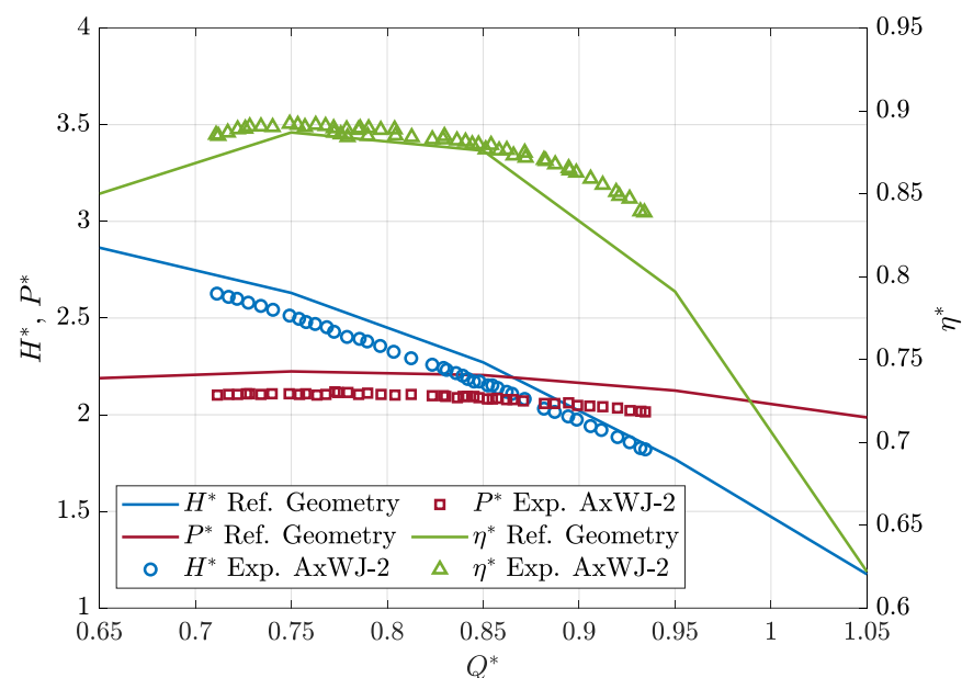
Figure 11. Predicted open-water performances of the reference geometry compared with experiments [50] of the original AxWJ-2 waterjet.
