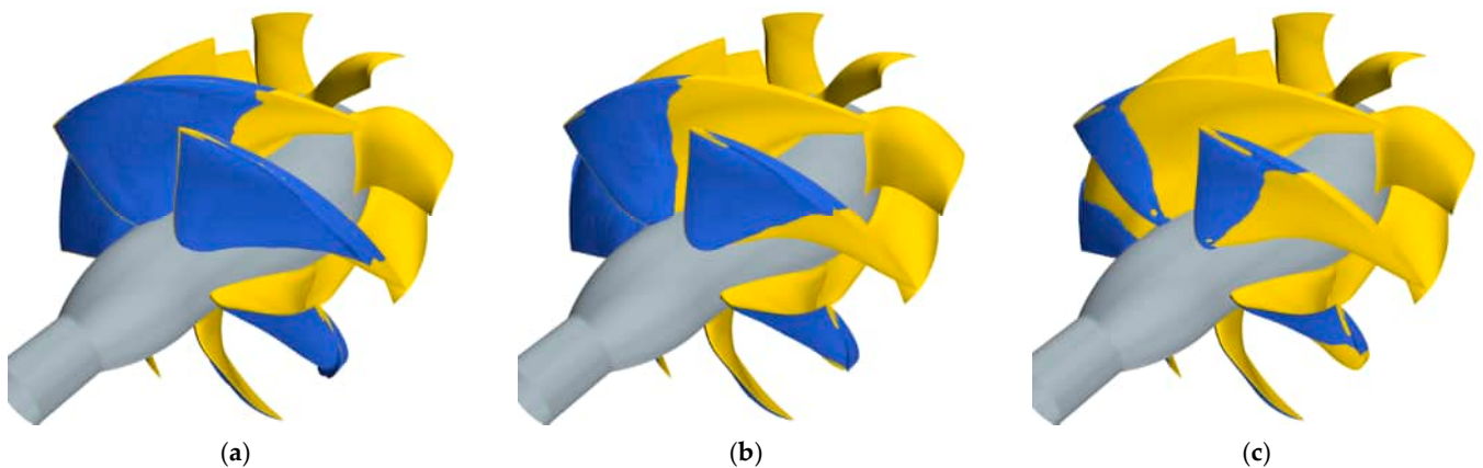
Figure 13. Predicted vapor bubble (isosurface of Vof = 0.5 ) for Q^* = 0.75 at \sigma_N = 4 (a), \sigma_N = 5 (b), and \sigma_N = 6 (c).
