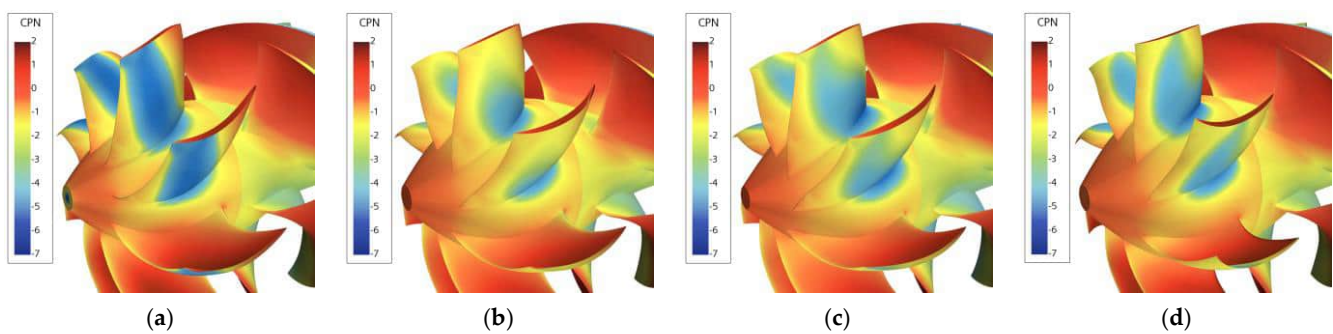
Figure 18. Pressure coefficient ( C_{PN} ) distributions over stator blades of the selected optimized waterjets. WJ-7801 (a), WJ-10128 (b), WJ-9400 (c), and WJ-4837 (d).
