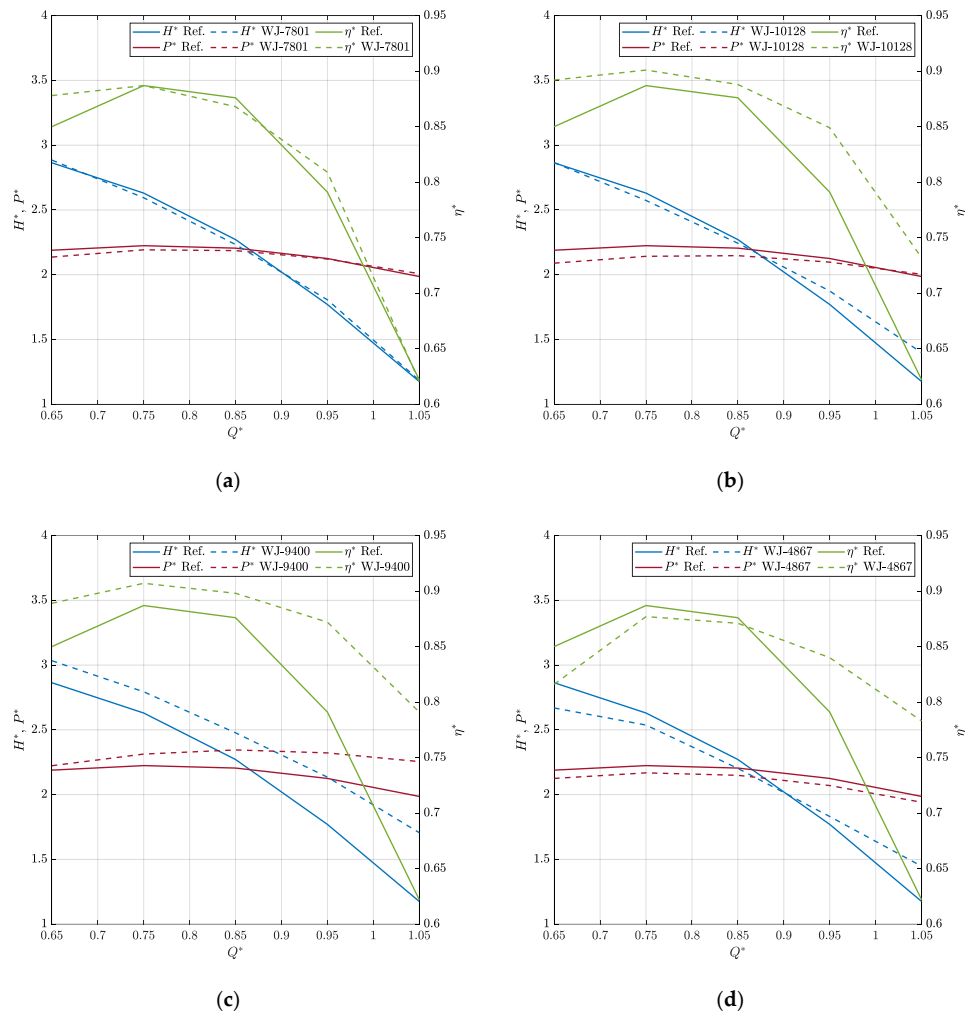
Figure 19. Non-cavitating performances of the selected waterjets. WJ-7801 (a), WJ-10128 (b), WJ-9400 (c), and WJ-4837 (d).
