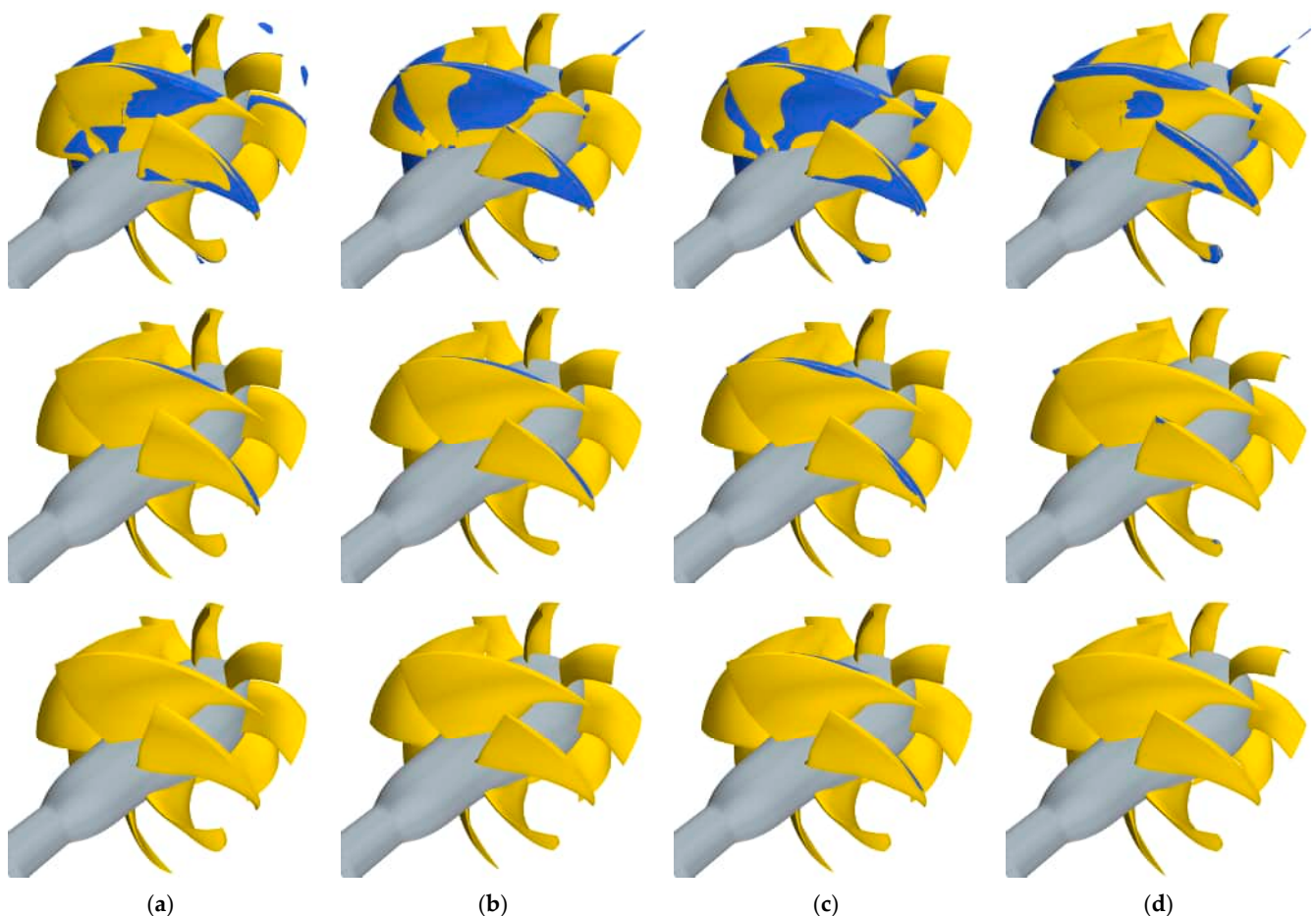
Figure 20. Predicted vapor bubble (isosurface of Vof = 0.5 ) for Q^* = 0.85 at \sigma_N = 4 ( top ), \sigma_N = 5 (intermediate), and \sigma_N = 6 ( bottom ) for the selected optimized waterjets. WJ-7801 ( a ), WJ-10128 ( b ), WJ-9400 ( c ), and WJ-4837 ( d ).
