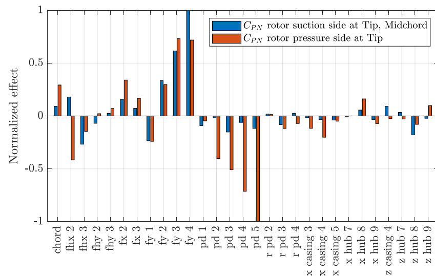
Figure 26. Effect (direct, positive, and inverse, negative) of factors (geometrical parameters of rotor, casing and hub) on the maximum value of the pressure coefficient on the suction side of the rotor, midchord at the tip, and on the maximum value of the pressure coefficient on the pressure side of the rotor at the tip.
