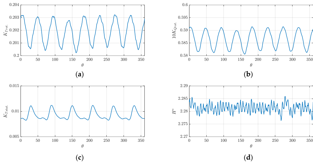
Figure 7. Unsteady performance ( Q^* = 0.85 ) of the reference axial waterjet. Unsteady rotor (single blade) thrust coefficient K_{T_{rot}} . (a), unsteady rotor (single blade) torque coefficient 10 K_{Q_{rot}} . (b), unsteady stator (single blade) thrust coefficient K_{T_{stat}} . (c), and unsteady head coefficient H^* (d).
