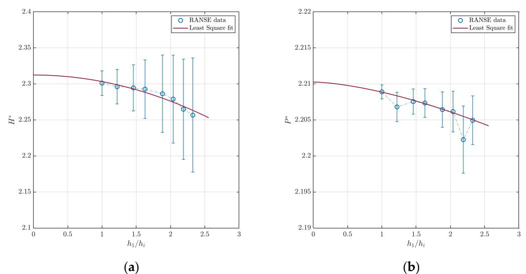
Figure 6. Grid sensitivity and associated numerical uncertainties: head (a) and power (b) coefficients under non-cavitating conditions ( Q^* = 0.85 ).
