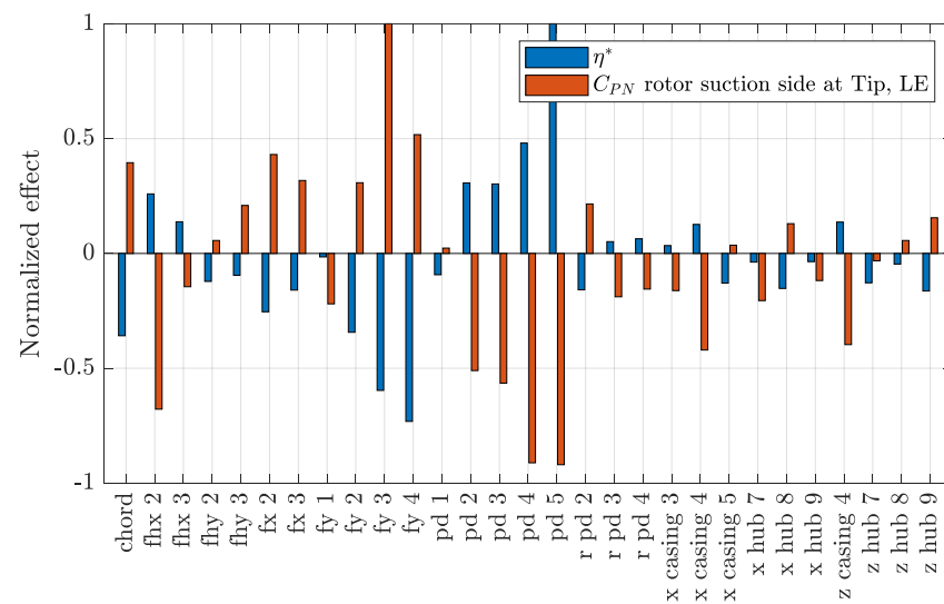
Figure 25. Effect (direct, positive, and inverse, negative) of factors (geometrical parameters of rotor, casing and hub) on efficiency and maximum value of the pressure coefficient on the suction side of the rotor, and the leading edge at the tip.
