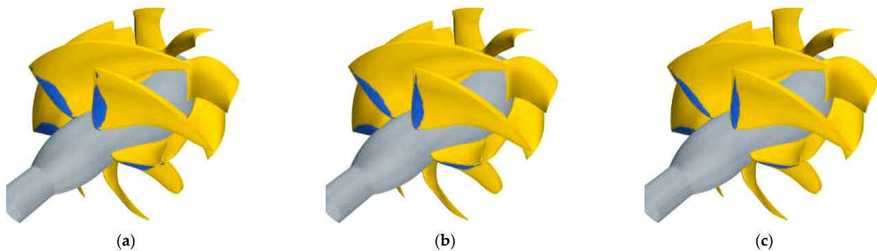
Figure 9. Predicted cavity bubble for different grid densities: coarsest h_1/h_i = 2.32 (a), intermediate h_1/h_i = 1.88 (b), and finest h_1/h_i = 1 (c) grid arrangements ( Q^* = 0.85 , \sigma_N = 5 ).
