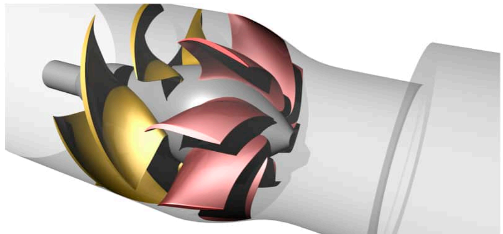
Figure 1. Geometry of the reference waterjet (modified AxWJ-2).
