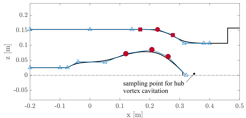
Figure 15. Parametric description of hub and casing using B-Spline polygons on the meridian plane. Control points marked with a circle can move in both x- and z-directions on the meridian plane. Control points marked with a square can move only along the x-direction.
