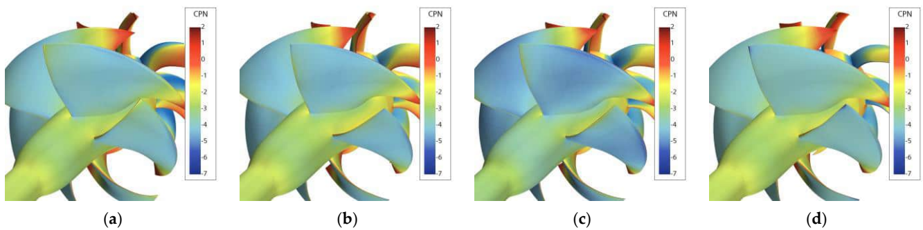
Figure 17. Pressure coefficient ( C_{PN} ) distributions over rotor blades of the selected optimized waterjets. WJ-7801 (a), WJ-10128 (b), WJ-9400 (c), and WJ-4837 (d).
