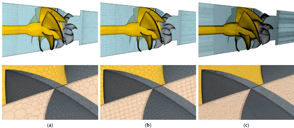
Figure 5. Computational grids and detail at the rotor tip for the grid sensitivity study: coarsest h_1/h_i = 2.32 (a), intermediate h_1/h_i = 1.88 (b), and finest h_1/h_i = 1 (c) grid arrangements.
