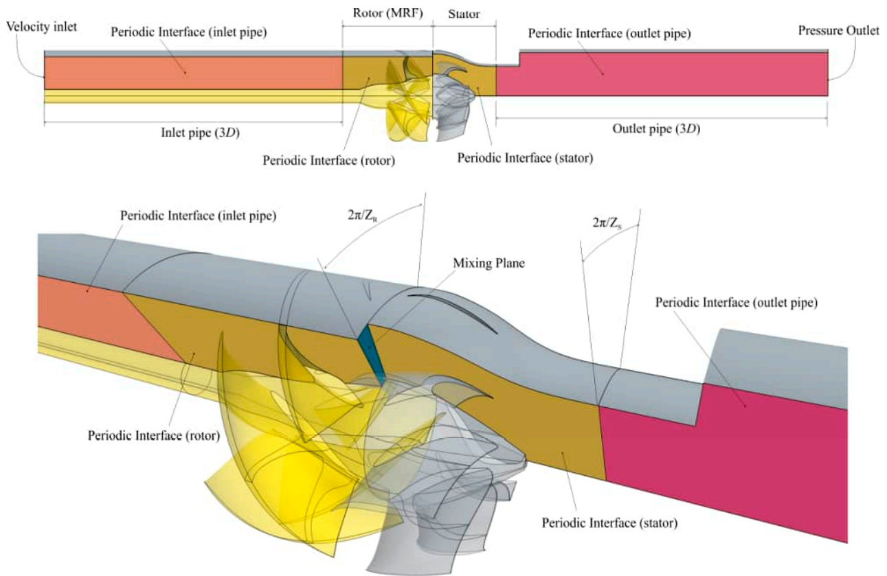
Figure 3. Computational domain and boundary conditions.
