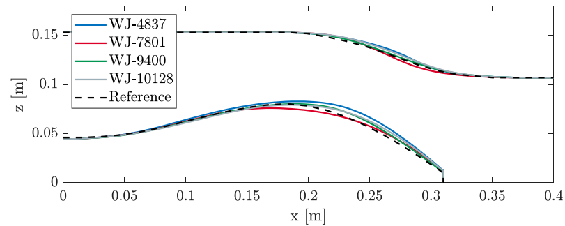
Figure 24. Blade passage (hub and casing meridian section) of selected optimized propellers.
