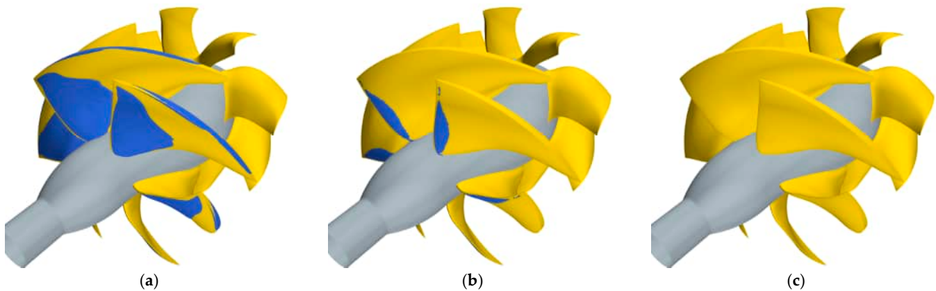
Figure 14. Predicted vapor bubble (isosurface of Vof = 0.5 ) for Q^* = 0.85 at \sigma_N = 4 (a), \sigma_N = 5 (b), and \sigma_N = 6 (c).
