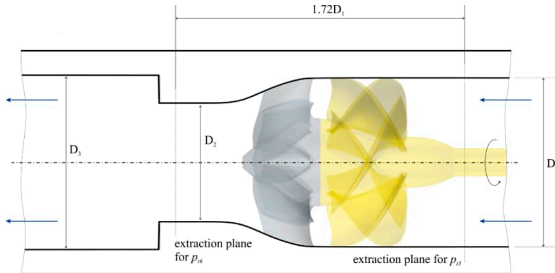
Figure 2. Reference for main dimensions and pressure sampling locations. More details are available in [7].
