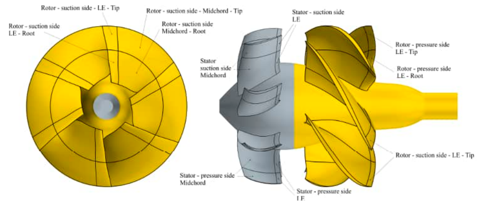
Figure 4. Rotor and stator blade patches subdivision for pressure sampling.
