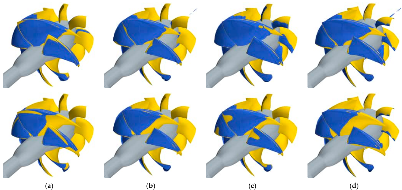
Figure 21. Predicted vapor bubble (isosurface of Vof = 0.5 ) for Q^* = 0.75 at \sigma_N = 4 (top), \sigma_N = 5 (bottom) for the selected optimized waterjets. WJ-7801 (a), WJ-10128 (b), WJ-9400 (c), and WJ-4837 (d).
