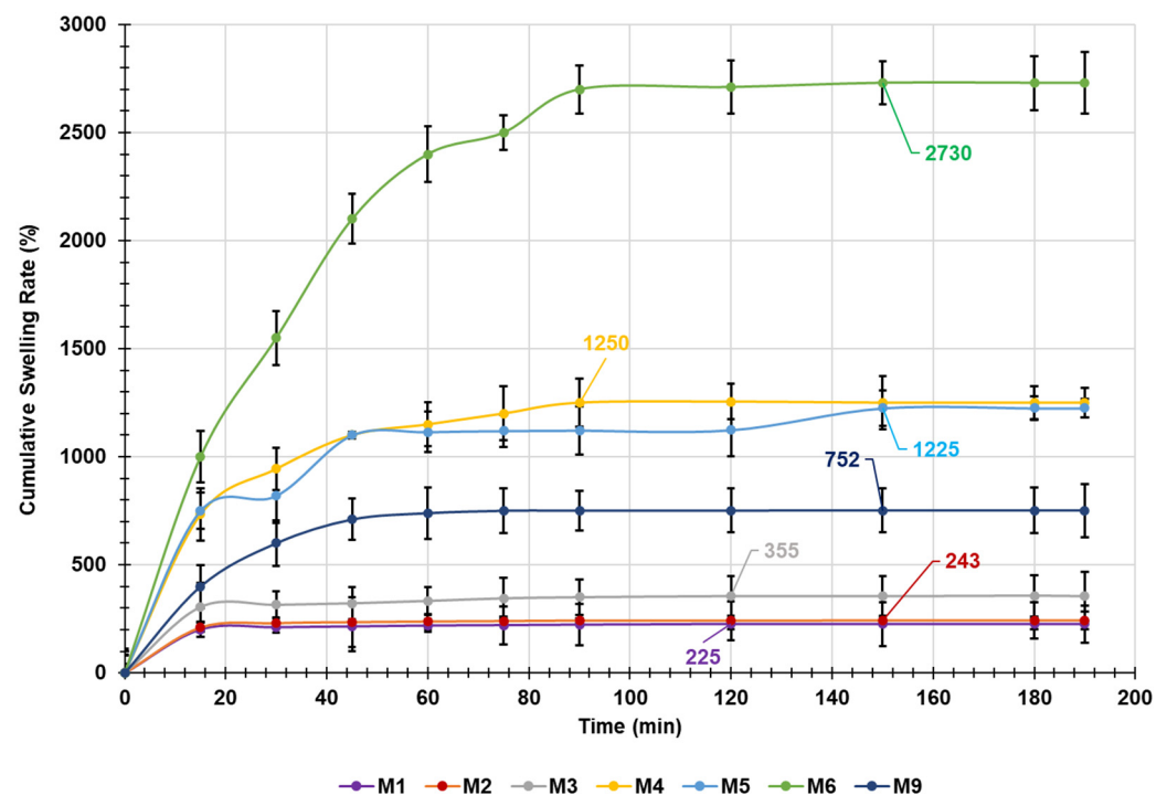
Figure 5. Plots of the cumulative swelling rate values of the crosslinked gelatines vs. time.
