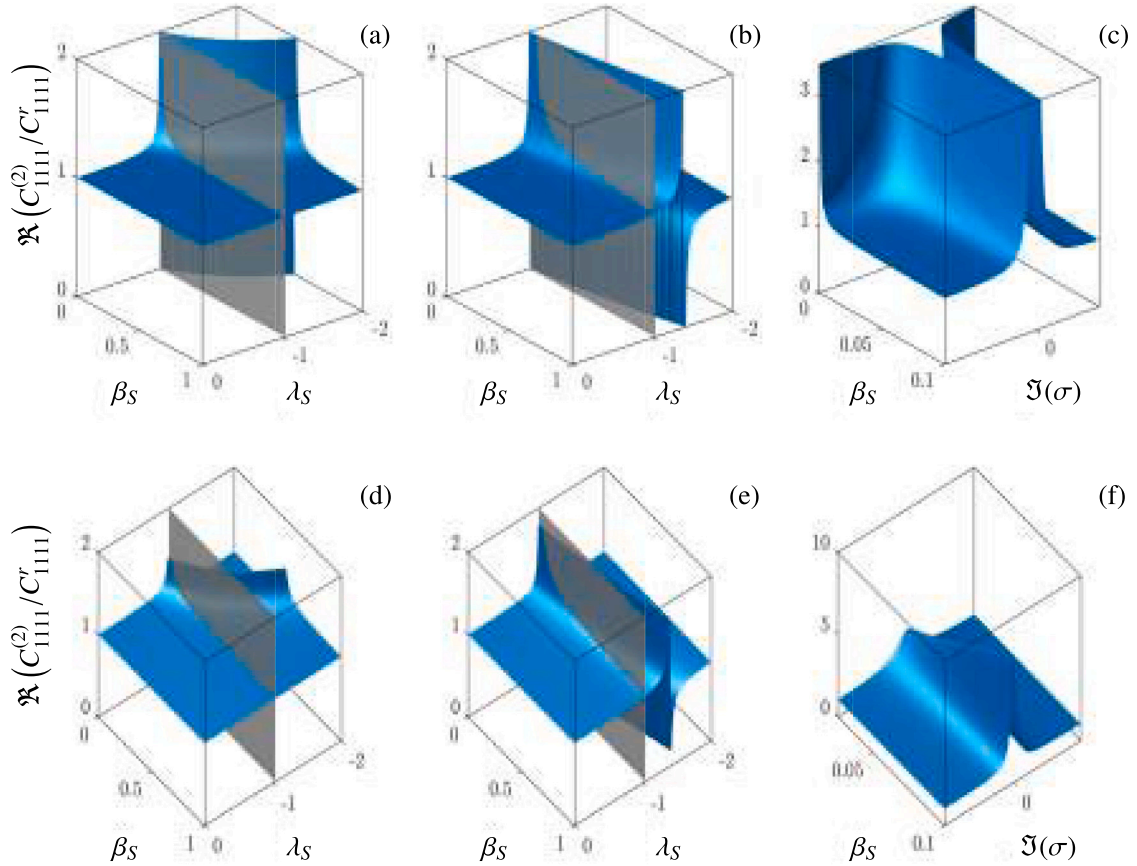
Fig. 3. A set of 3D surface plots of \text{Re}(C_{1111}^{(2)}(\lambda_S, \alpha_S, \beta_S, \gamma)) in the parameters space.
