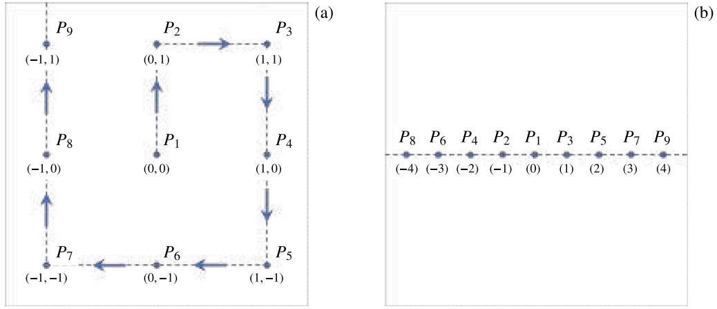
Fig. 2. (a) Spiral ordering of points identified by the 2D-index \mathbf{m} = (m_1, m_2) ; (b) Linear ordering of the 1D-index \mathbf{m} = (m_1) as a result of the linearization procedure.
