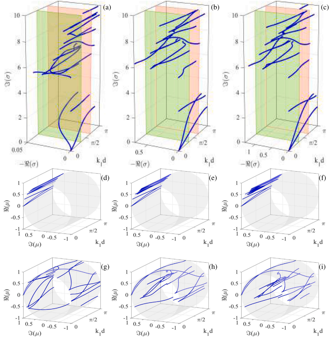
Fig. 8. Dispersion curves for \alpha_S = 10^{-3} , and \lambda_S = \lambda_R as \beta_S varies. (a), (b), (c) Complex Floquet-Bloch spectra for \beta_S = 10^{-i} , i = 3, 4, 5 , respectively. (d), (e), (f) dispersion curves in terms of \mu on the unit cylinder for \tau=0.1 ; (g), (h), (i) dispersion curves in terms of \mu on the unit cylinder for \tau=1 .
