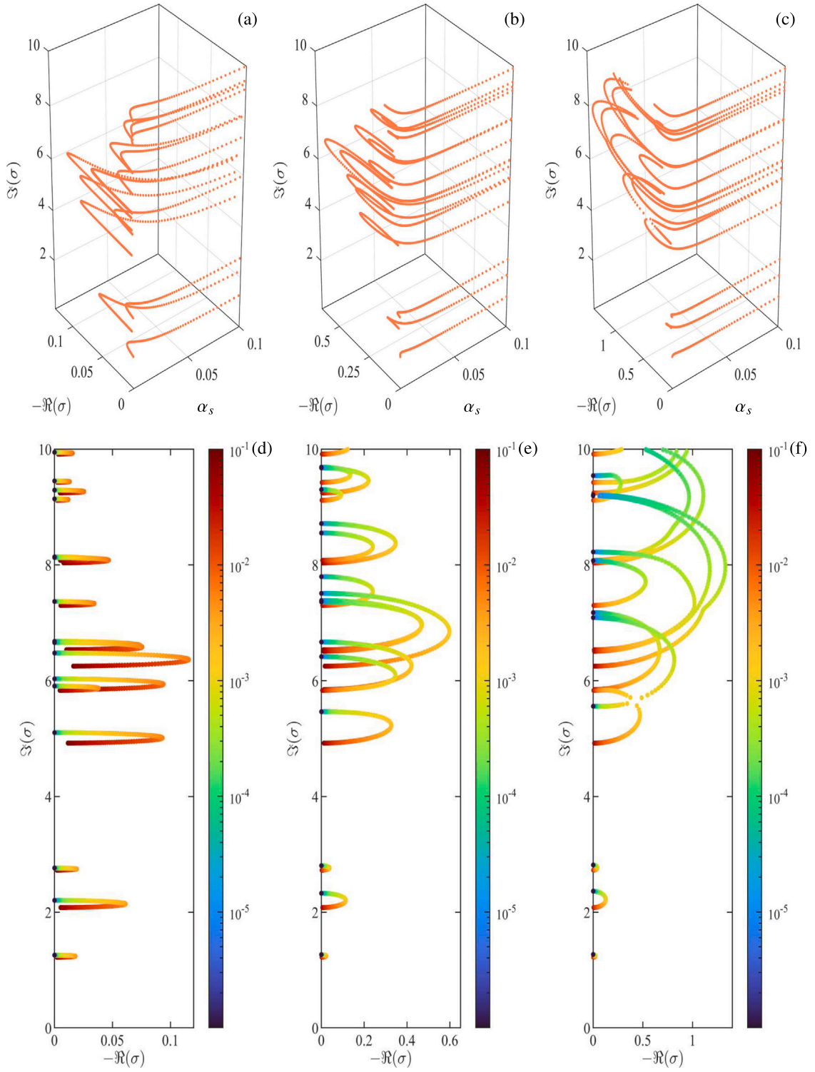
Fig. 12. Loci of the complex frequency for k_1 d = 2\pi/3 : (a), (b), (c) 3D plots of real and imaginary parts of the dimensionless complex frequency \sigma versus \alpha_s for \beta_s = 10^{-i} , i = 3, 4, 5 , respectively; (d), (e), (f) 2D plots of real and imaginary parts of the dimensionless complex frequency \sigma with \alpha_s shown as a logarithmic colour scale.
