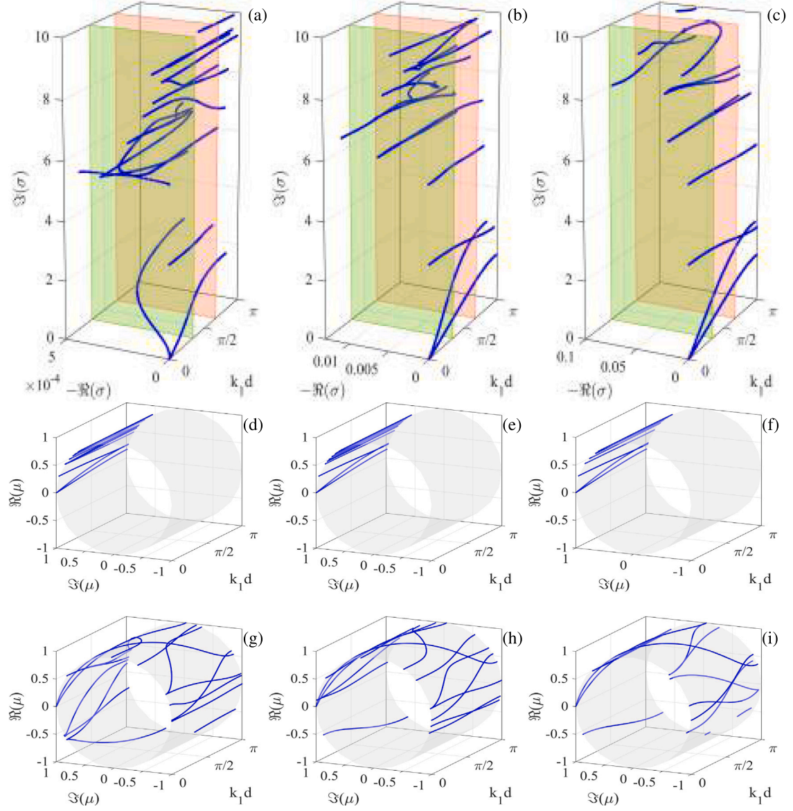
Fig. 6. Dispersion curves for \alpha_S = 10^{-5} , and \lambda_S = \lambda_R as \beta_S varies. (a), (b), (c) Complex Floquet-Bloch spectra for \beta_S = 10^{-i} , i = 3, 4, 5 , respectively. (d), (e), (f) dispersion curves in terms of \mu on the unit cylinder for \tau=0.1 ; (g), (h), (i) dispersion curves in terms of \mu on the unit cylinder for \tau=1 .
