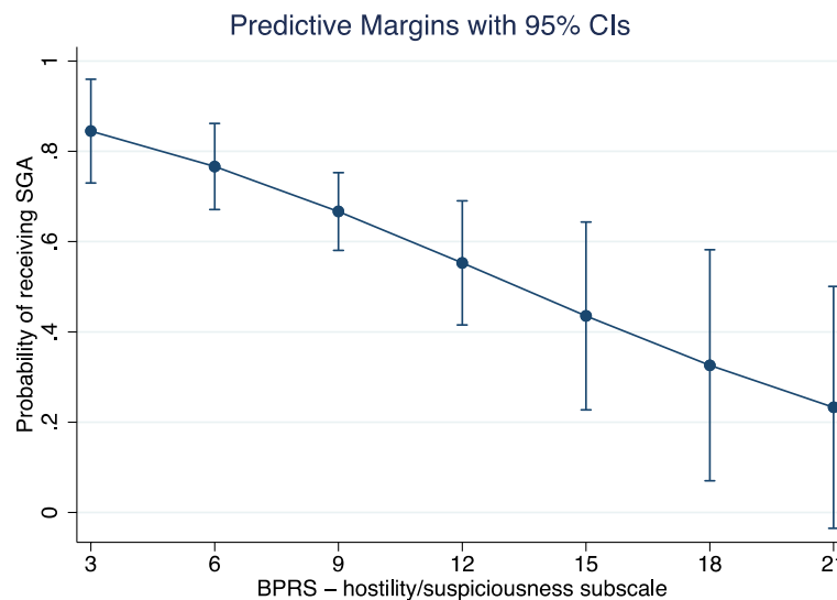
Fig. 2 Likelihood of receiving an SGA based on BPRS hostility score. The larger confidence interval suggests greater uncertainty for higher scores
