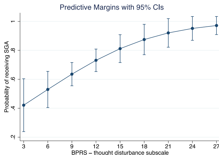
Fig. 1 Likelihood of receiving an SGA based on BPRS thought disturbances score. The larger confidence interval suggests greater uncertainty for lower scores
