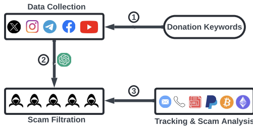
Figure 1: Evaluation Setup Design: An overview of our system, which consists of mainly three components: (i) Data Collection which performs automated donation-based keyword searches in five social media platforms, (ii) Scam Filtration which performs data filtration associated to donation soliciting fraudulent accounts, and (iii) Tracking and Scam Analysis which provides an evaluation of scammer’s modes of operation and techniques.
