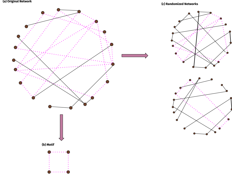
Figure 7: Example of motifs in a toy network. Looking at the original network (a) it is clear that the “squared” subgraph (b) ( G_5 in Figure 4) is over represented in the original network w.r.t. randomized versions of it (c).
