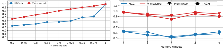
Figure 43: Comparison of TAGM with its extensions in terms of V-measure and MCC. On the left hand panel we drew the ratio V\text{-measure}(\text{TAGM})/V\text{-measure}(\text{IncTAGM}) and the ratio MCC(\text{TAGM})/MCC(\text{IncTAGM}) as the percentage of training data increases. On the right hand panel we drew the V-measure and MCC of MemTAGM and TAGM as the memory of the hidden Markov process increases.
