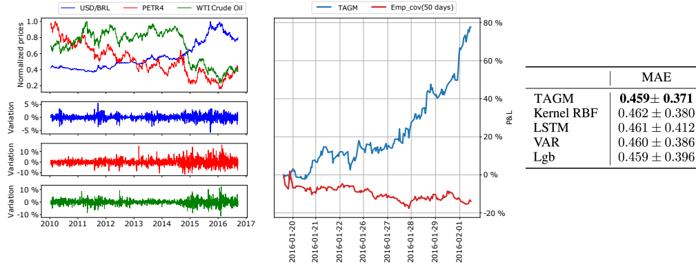
Figure 45: TAGM enables significant improvement in the construction of a financial portfolio (central panel) due to its ability to promptly detect changes in underlying dependencies among stocks (data showed on the left). TAGM shows better performance also in the prediction of next day stock prices (right panel).
