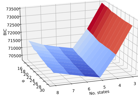
Figure 46: Cross validation
