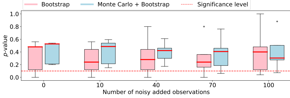
Figure 15: Results in terms of p -values for the two testing pipelines as the input data present an increasing level of noisy observations.
