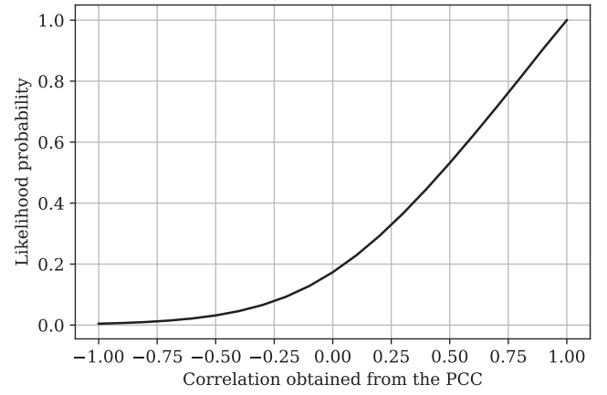
Fig. 1. Representation of Eq. (12) in which the relationship between the PCC and the likelihood probability is obtained.
