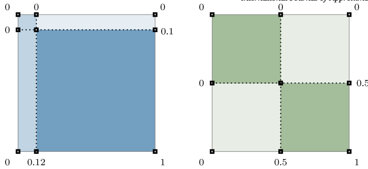
Fig. 2. Left: A representation of the grid domain U_2 \times V_2 , support of the discrete copula C_1 . Right: The grid support I_2 \times I_2 of the discrete copula \bar{C}_1 with the same dependence structure of C_1 . The colors represent a heatmap of the corresponding probabilities.
