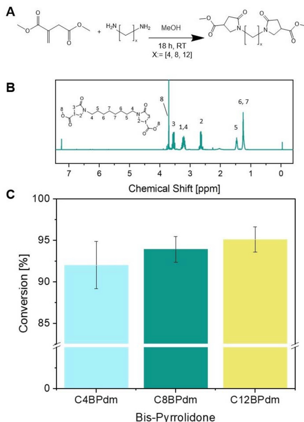
Fig. 2 Synthesis of the bis-pyrrolidone (CxBPdm) building blocks. (A) The reaction between DMI and diamine spacers with x : = [4, 8, and 12] using a catalytic amount of methanol used to prepare the BPdm structures. (B) 1 H-NMR spectrum of C8BPdm; (C) the raw yield of BPdm structures (calculated using eqn (1)).
