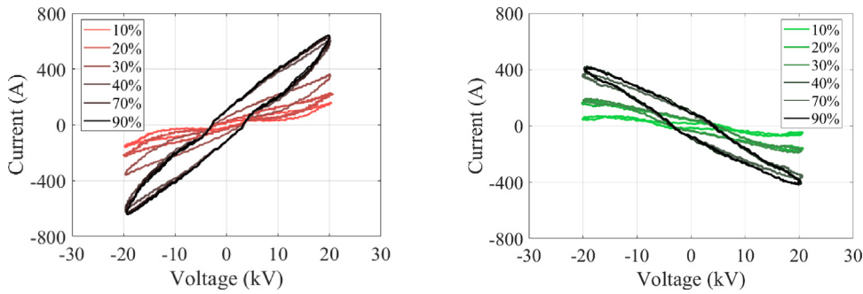
Fig. 1. VI diagrams at various percentages of absorbed current measured with respect to the nominal value of the Swiss locomotive Re460: traction (left), braking (right).
