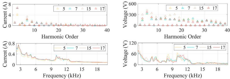
Fig. 14. Spectra patterns for clusters 5, 7, 15 and 17 of France data (50 Hz fundamental): harmonics current (top left), harmonic voltage (top right), supraharmonic current (bottom left), and supraharmonic voltage (bottom right).
