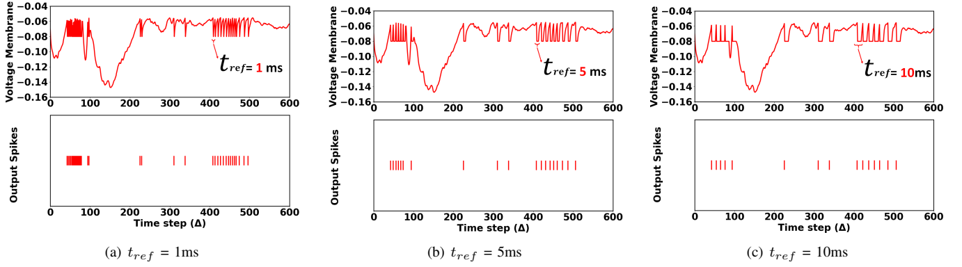
Fig. 4. Impact of changing the t_{ref} on the behavior of the voltage membrane potential and spiking activity of the LIF neuron using the same raw input. a) t_{ref} = 1 \text{ ms} (spike count = 38), b) t_{ref} = 5 \text{ ms} (spike count = 19), and c) t_{ref} = 10 \text{ ms} (spike count = 15). (Top): voltage membrane dynamics of the LIF neuron. (Bottom): raster plot or spiking activity of the LIF neuron.
