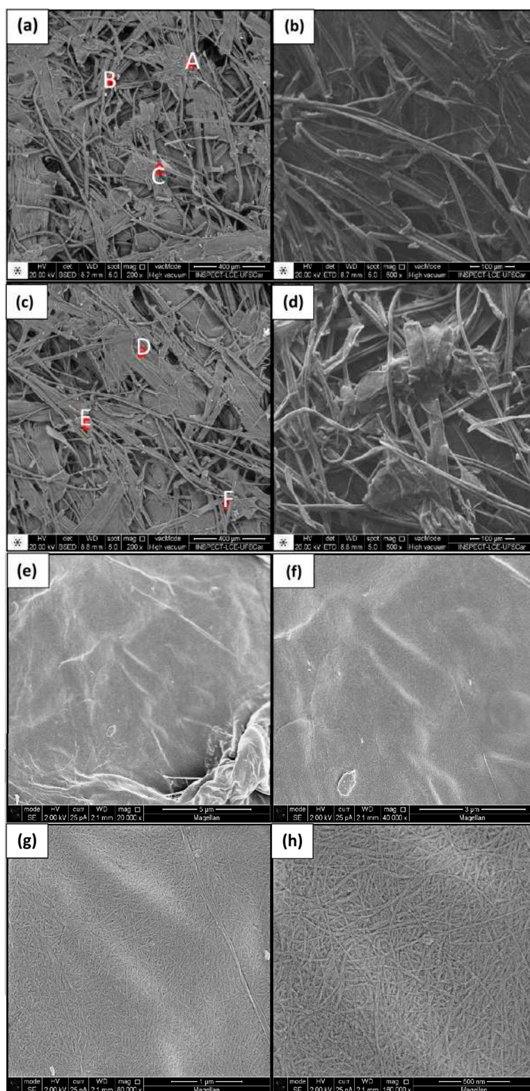
Figure 8. Micrographs of sugarcane bagasse at magnification of (a) 200 \times , (b) 500 \times , (c) 200 \times , (d) 500 \times , (e) 20 k \times , (f) 40 k \times , (g) 80 k \times , (h) 160 k \times . Samples chosen for the EDS analysis were taken from points A, B, C, D, E and F.
