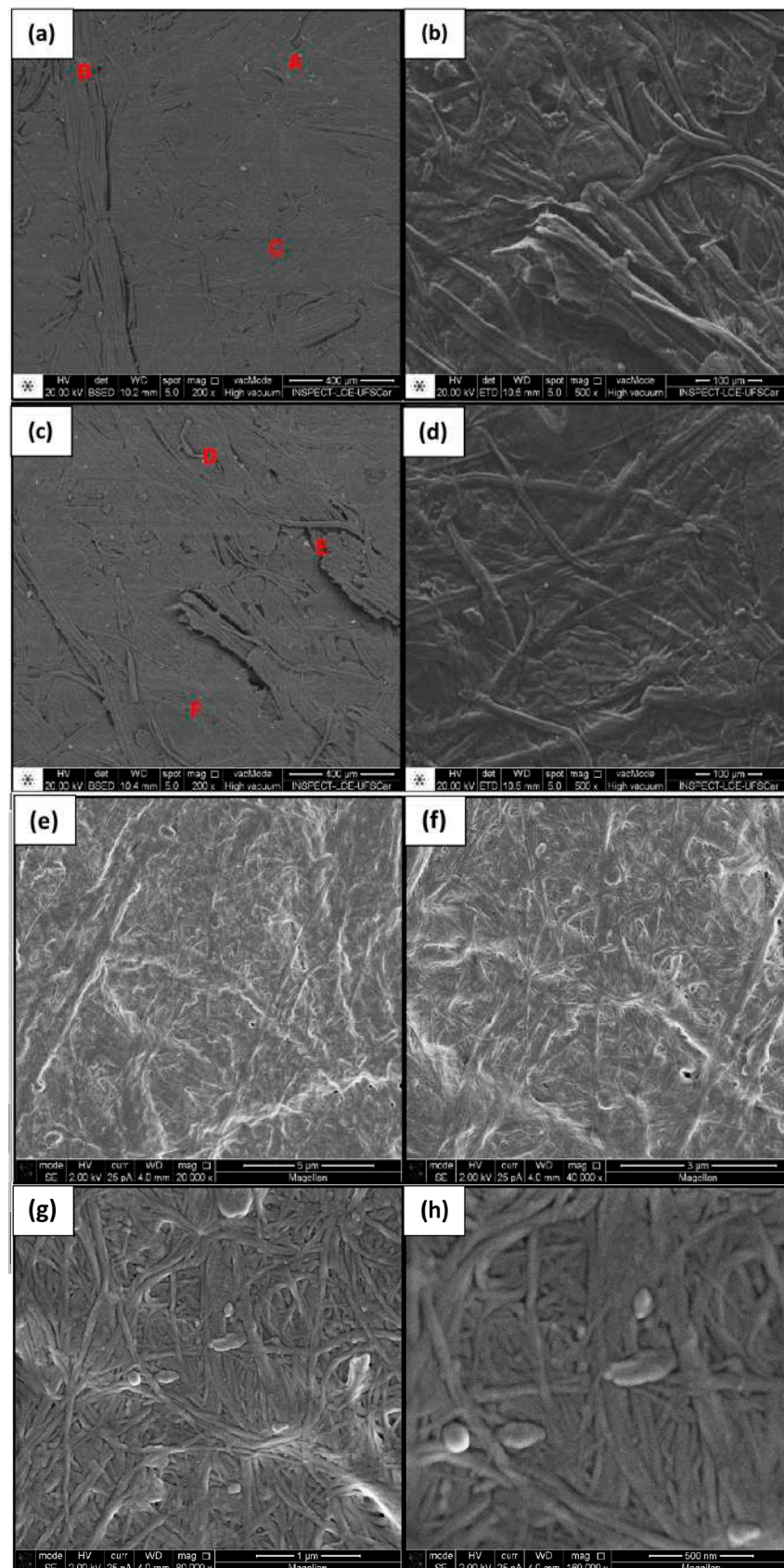
Figure 9. Micrographs of the BC/SCB composite, composed of 50% ( w/w ) bacterial cellulose plus 50% ( w/w ) sugarcane bagasse, with magnification of (a) 200×, (b) 500×, (c) 200×, (d) 500×, (e) 20 k×, (f) 40 k×, (g) 80 k×, (h) 160 k×. Samples chosen for the EDS analysis were taken from points A, B, C, D, E and F.
