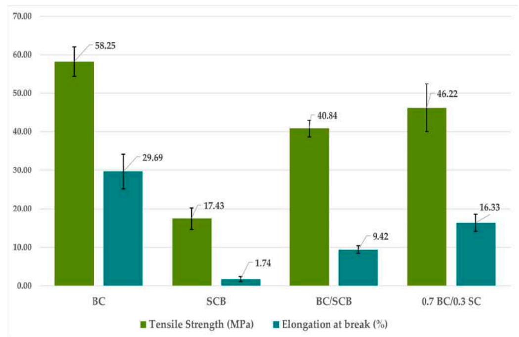
Figure 12. Graph of tensile strength (MPa) and elongation at break (%) of bacterial cellulose (BC) and sugarcane bagasse (SCB) samples. BC = BC alone, SCB = SCB alone, BC/SCB = 50% ( w/w ) BC plus 50% ( w/w ) SCB, 0.7 BC/0.3 SCB = 70% ( w/w ) BC plus 30% ( w/w ) SCB.
