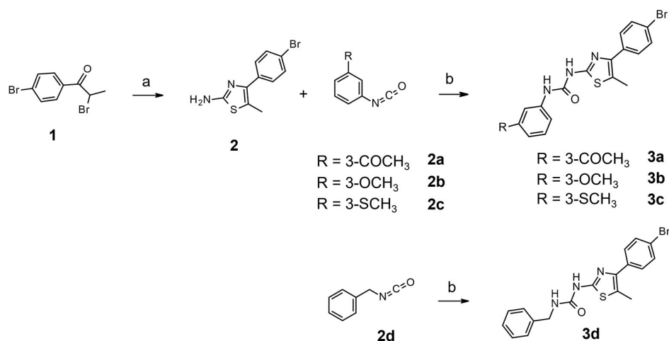
Scheme 1. Reagents and conditions: (a) thiourea, ethanol, reflux, 6 h; (b) anhydrous acetonitrile, 80^\circ\text{C} for 3 h then room temperature for 1 h.
