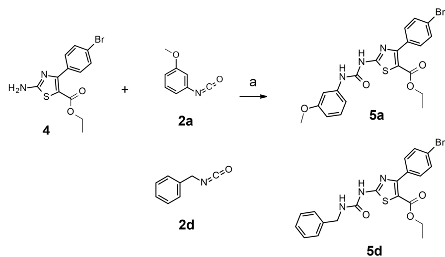
Scheme 2. Reagents and conditions: (a) anhydrous acetonitrile, 80^\circ\text{C} for 6 h.
