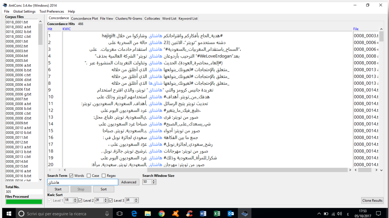
Figura 36 - analisi del prestito هاشتاق hāštāq "hashtag": in AntConc: Cluster.
