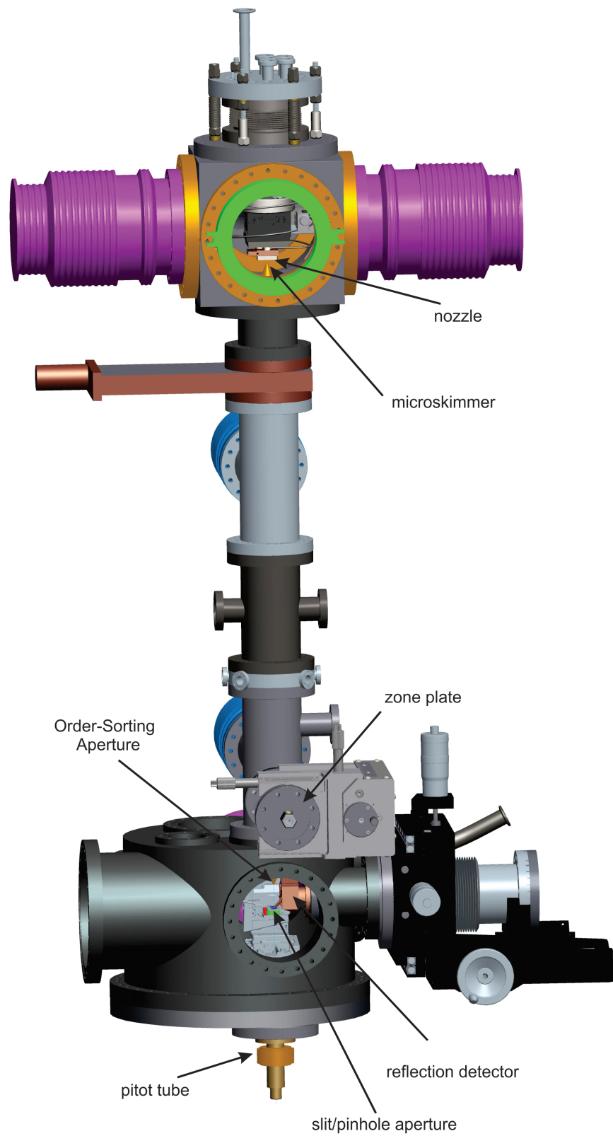
FIG. 1. Drawing of instrument NEMI used to perform the measurements presented here. The focused helium atom spot profile is observed by moving a 10\ \mu\text{m} slit aperture, mounted on a translation stage, across the focused spot and measure the pressure increase in the Pitot tube detector. To the right the detector setup used for reflection imaging can be seen. It is not used for the experiments presented here.
