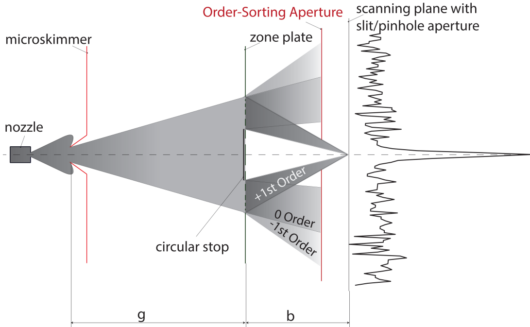
FIG. 2. Diagram of the 0-order filter setup. After the free-jet expansion through the nozzle, the central part of the helium beam is selected by the microskimmer. The beam hits the Fesnel zone plate (ZP). The central part of the zone plate has been blocked by a circular middle stop which filters part of the 0-order beam. The rest of the 0-order beam (and most of the higher orders) is blocked by the order-sorting aperture with a diameter slightly smaller than the middle stop.
