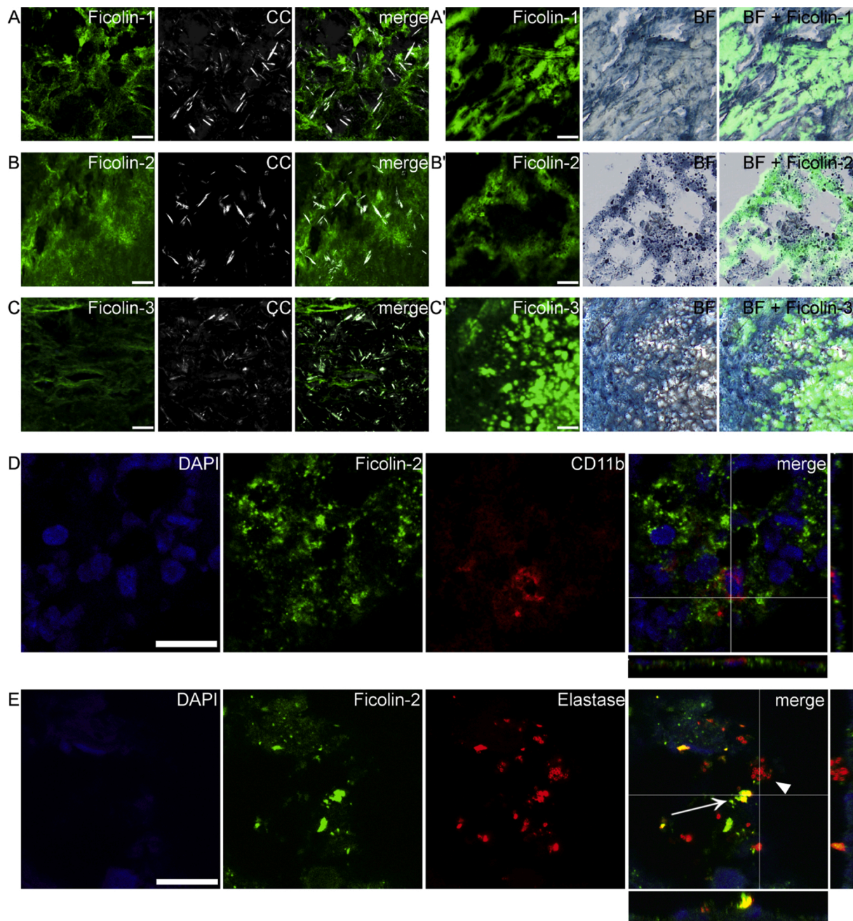
Fig. 2. Intraplaque localization of ficolins. Ficolin-1 (A), -2 (B) and, to a lesser extent, -3 (C, green) were present in necrotic core areas enriched in cholesterol crystals (CC, white). All ficolins were also present in calcified parts of the plaques visible at brightfield microscopy (BF, A', B' and C'). Scale bars 50 μm. Panel D shows ficolin-2 (green) surrounding macrophages (CD11b, red) recruited to the plaques' necrotic core. Panel E shows ficolin-2 (green) and neutrophils' elastase (red) in the necrotic core. Few neutrophils appeared positive for ficolin-2 (arrow), but the majority of them was located in areas negative for ficolin-2 (arrowhead). Scale bars 20 μm.
