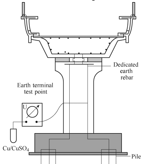
Fig.3 Average potential shift of structure
