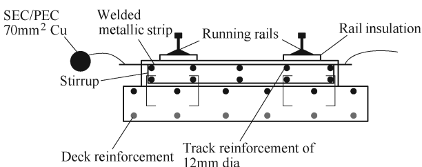
Fig.17 Case (1) cross-section
