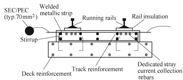
Fig.18 Case (2) cross-section
