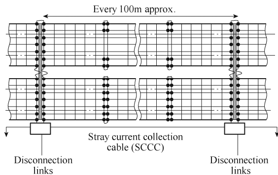
Fig.10 Floating SCCS interconnection
