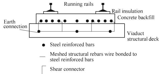
Fig.13 Earthed SCCS
