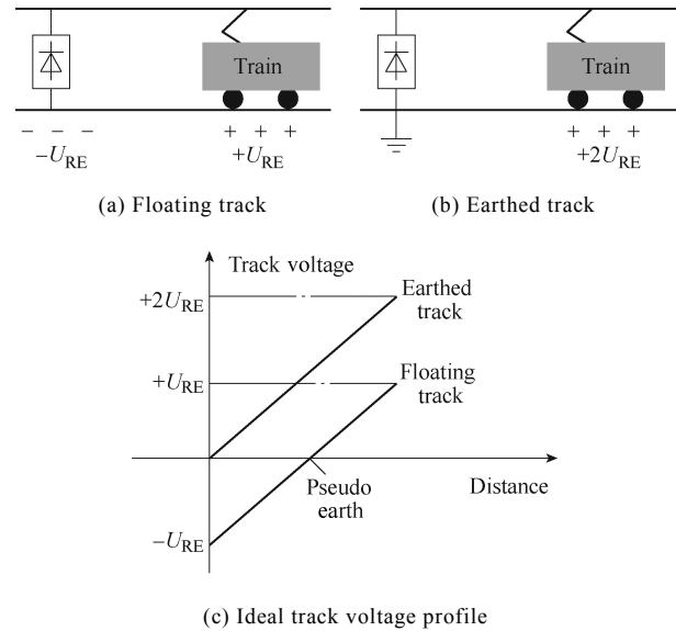
Fig.5 Diagram of rail potential profile
