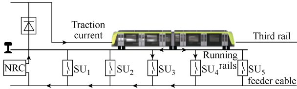
Fig.21 NRC traction power system
