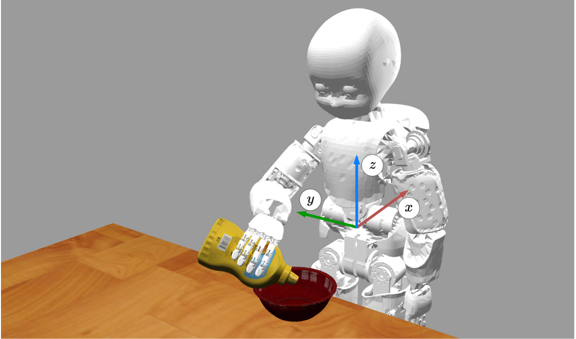
Figure 4.6 The iCub robot in the Gazebo environment. The root frame attached to the robot is also depicted.
