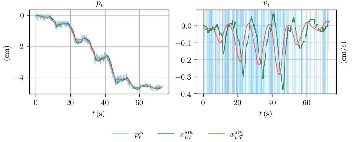
Figure 6.5 On the left, a comparison between the ground-truth position from the ArUco marker detection system p_t^A , its filtered version x_{t|t}^{sm} and its smoothed version x_{t|T}^{sm} obtained using a Kalman filter and smoother respectively. On the right, comparison between the ArUco velocity signal obtained using finite differences, filtered and smoothed version.
