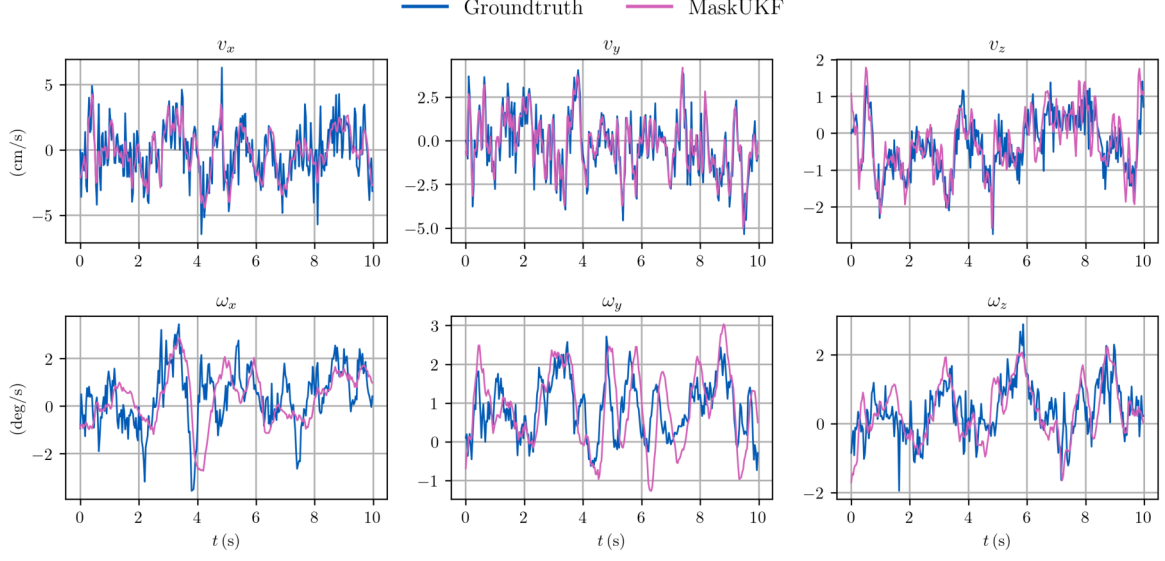
Figure 4.4 Comparison between the estimated linear velocity v^m and angular velocity \omega and the ground truth velocities within a video sequence from the YCB-Video dataset. The ground truth velocities are obtained from finite differences.
