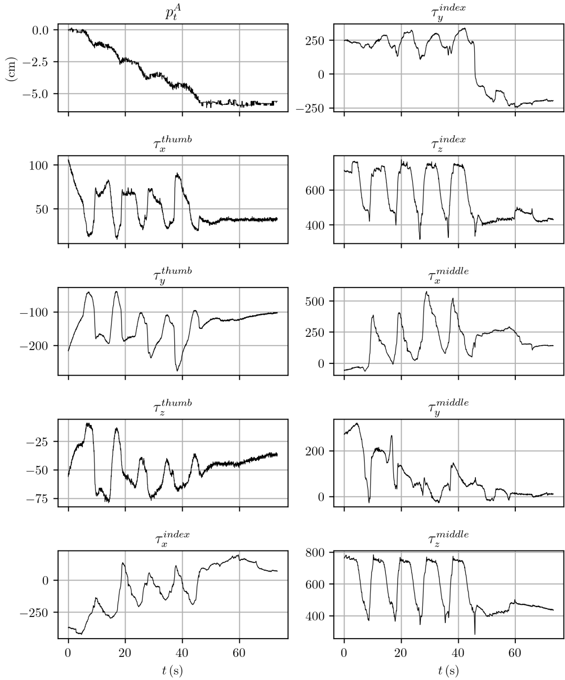
Figure 6.8 Data traces for one of the data collection experiment performed using the mustard bottle. The tactile signals correspond to the raw sensor reading using arbitrary units.
