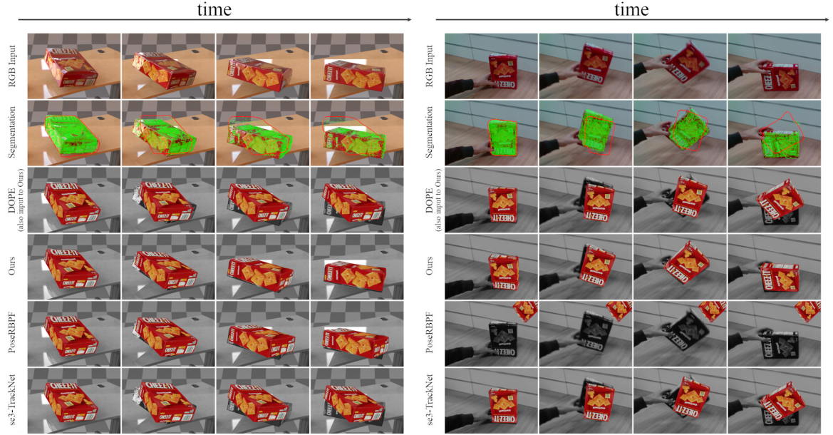
Figure 5.4 Qualitative results for the object cracker box (003). On the left: frames from Fast-VCB. On the right: frames acquired with a RealSense D415 camera. The time length of the object motion is approximately 1 second. The red contour in the Segmentation row represents the stream of delayed masks M_t^d , the green dots represent the masks M_t propagated using the optical flow.
