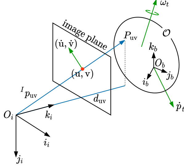
Figure 3.4 Representation of the vector {}^I p_{uv} from the origin O_i to the point P_{uv} belonging to the object \mathcal{O} , the depth d_{uv} , i.e. the z coordinate of the vector, and the projection of the vector onto the image plane, corresponding to the pixel coordinates (u, v) . The object linear velocity \dot{p}_t and angular velocity \omega_t , and the corresponding velocity of the pixel location (\dot{u}, \dot{v}) are also represented.
