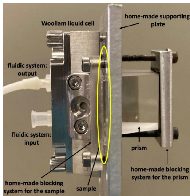
Figure 3.11 – SPEE set-up: focus on the blocking system of the sample.
