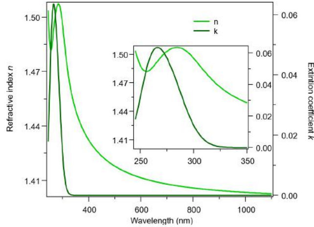
Figure 4.15 – Refractive index and extinction coefficient related to the GenOsc layer representing FZ24 dsDNA/MCH SAMs ( n(1300\text{ nm})=1.40 ) (dashed lines in Figure 4.14).
