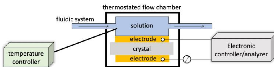
Figure 2.25 – Scheme of a QCM-D set-up.
