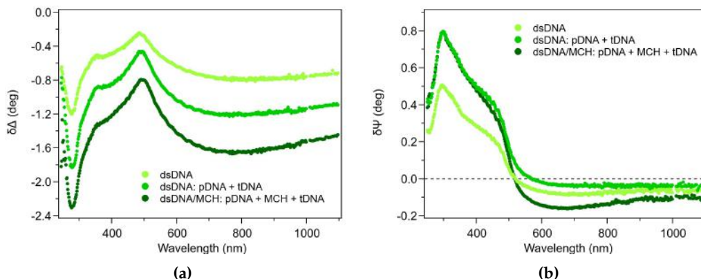
Figure 4.36 – dsDNA films: comparison between SE spectra of dsDNA/MCH SAMs (pDNA + MCH + tDNA)(dark green) and dsDNA films prepared by incubation in dsDNA solution (light green) or in pDNA and then in tDNA (green). (a) \delta\Delta and (b) \delta\Psi spectra.
