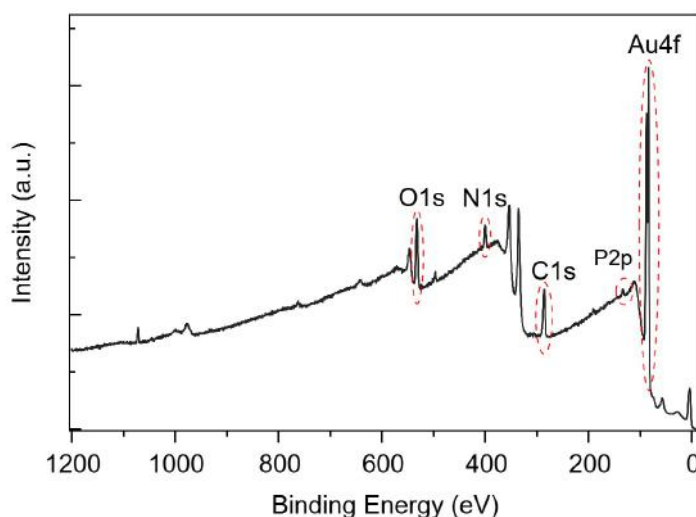
Figure 4.20 – XPS survey referred to dsDNA/MCH SAMs.
