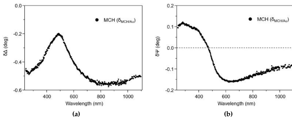
Figure 4.8 – MCH films on gold: SE experiment. (a) \delta\Delta and (b) \delta\Psi spectra obtained after 1 hour deposition in 5 \mu M MCH solution in 1 M NaCl TE buffer.
