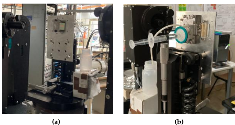
Figure 3.12 – Set-up for in situ SPEE experiments using the Woollam liquid cell and the W-VASE ellipsometer.
