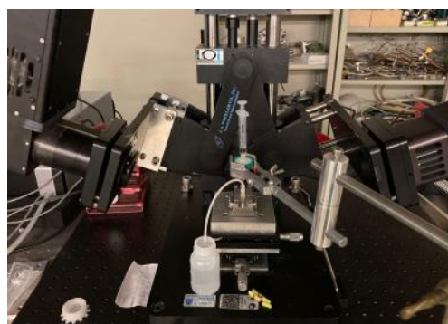
Figure 3.9 – Set-up for in situ SE experiments using Woollam liquid cell.
