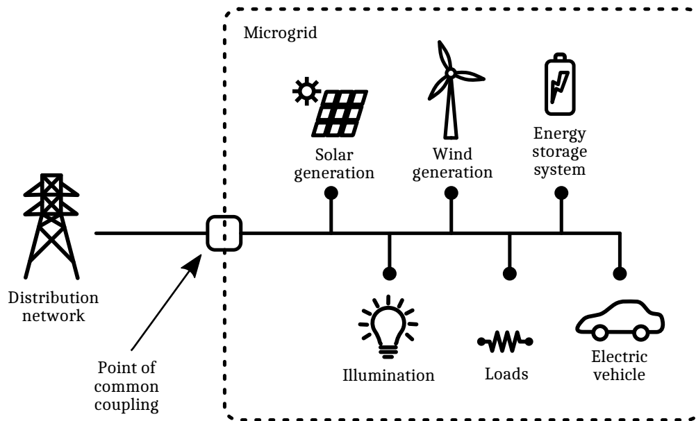
Figure 2.3: Basic structure of a microgrid.
