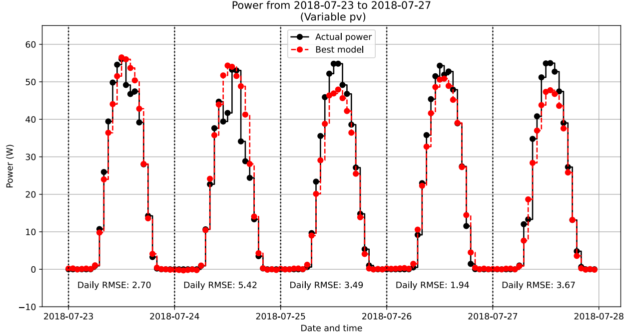
Figure 5.7: Example of deterministic forecasting for the variable pv .
