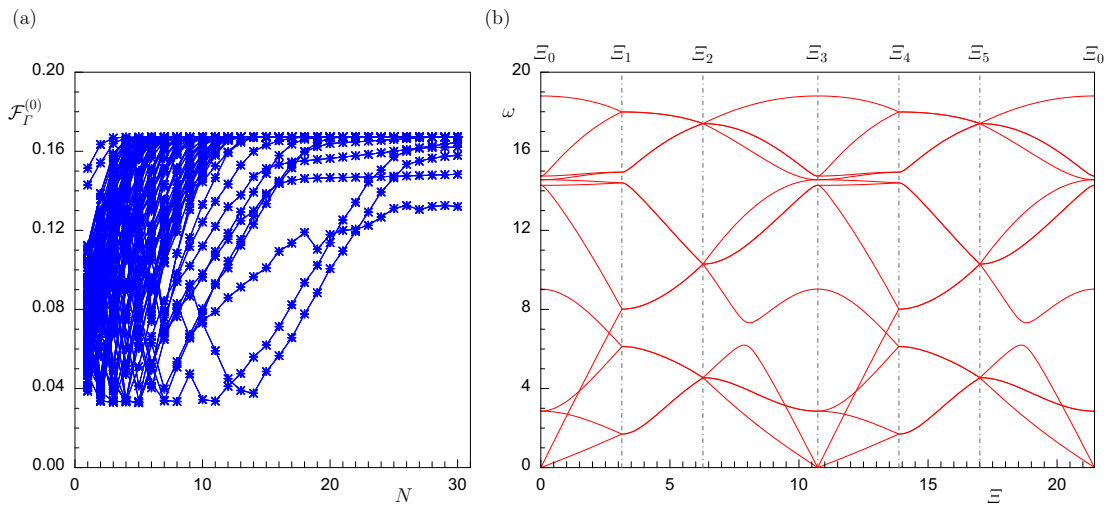
Figure 4: First optimization scenario for the Case C_0 : (a) converging objective values vs the iteration number for different GCMMA repetitions, (b) dispersion curves of the optimized spectrum.
