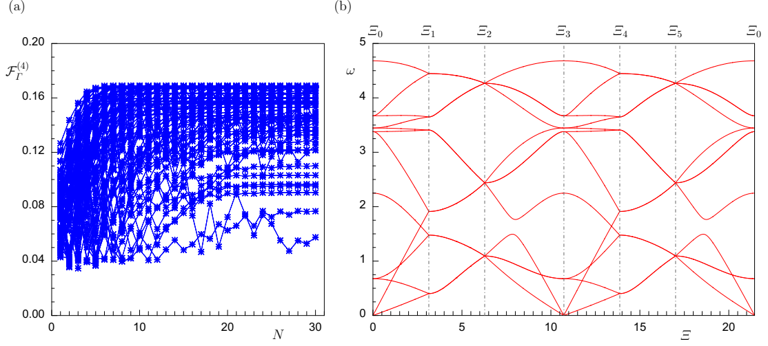
Figure 9: First optimization scenario for the Case C_4 : (a) converging objective values vs the iteration number for different GCMMA repetitions, (b) dispersion curves of the optimized spectrum.
