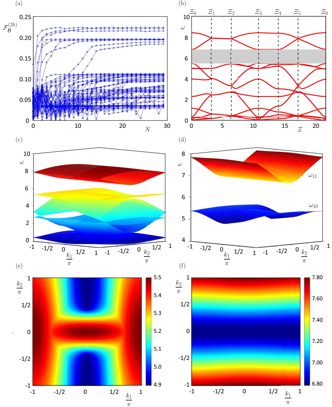
Figure 6: First optimization scenario for the Case C 2h : (a) converging objective values vs the iteration number for different GCMMA repetitions, (b),(c) dispersion curves and surfaces of the optimized spectrum, (d) optimal band gap, (e),(f) 10th and 11th dispersion surfaces in the \mathcal{B} -space.
