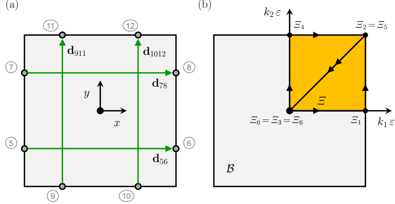
Figure 2: Periodic square cell: (a) central reference system and periodicity vectors, (b) whole first Brillouin zone \mathcal{B} and \mathcal{E} -coordinate spanning the closed polygonal curve \Gamma .
