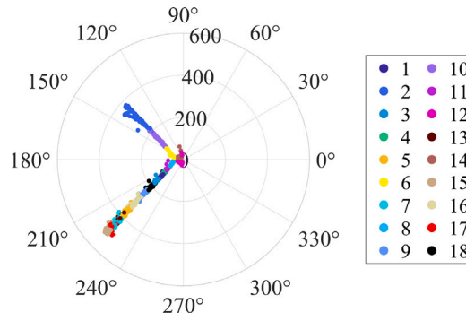
Fig. 13. Fundamental frequency (50 Hz, France) polar plot by sample and cluster color.
