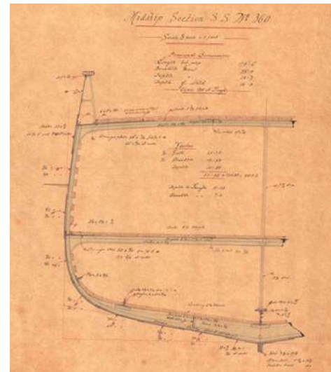
S.S. N 360, Midship section, china nera su lucido marrone acquarellata, Archivio DuilioShip
