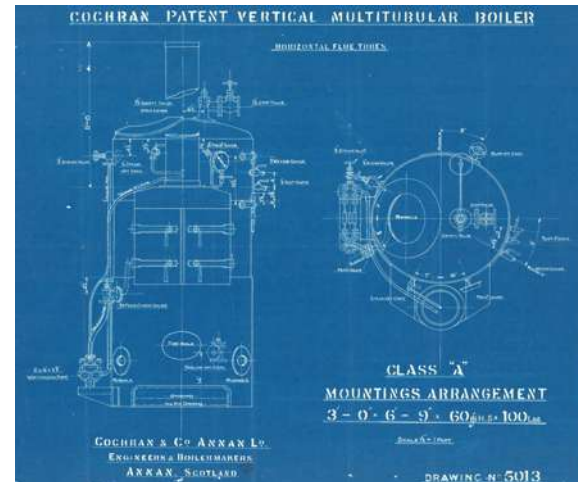
Cochran Patent Vertical Multitubular Boiler, blueprint Cochran & Co., Annan, Ltd, Scotland, Archivio DuilioShip
