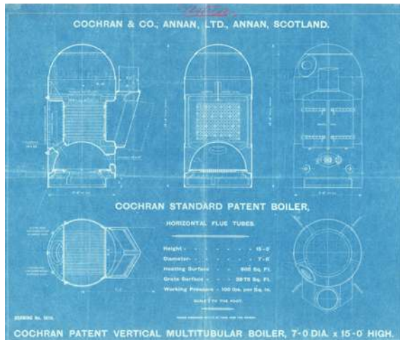
Cochran Standard Patent Boiler, Horizontal Flue Tubes, blueprint Cochran & Co., Annan, Ltd., Scotland, Archivio DuilioShip
