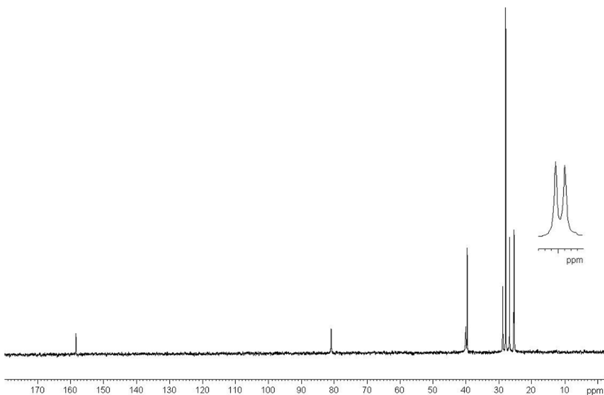
Figure S11. ^{13}\text{C} NMR ( \text{D}_2\text{O} , 75.5 MHz) spectrum of the hydrochloride salt of 6c .
