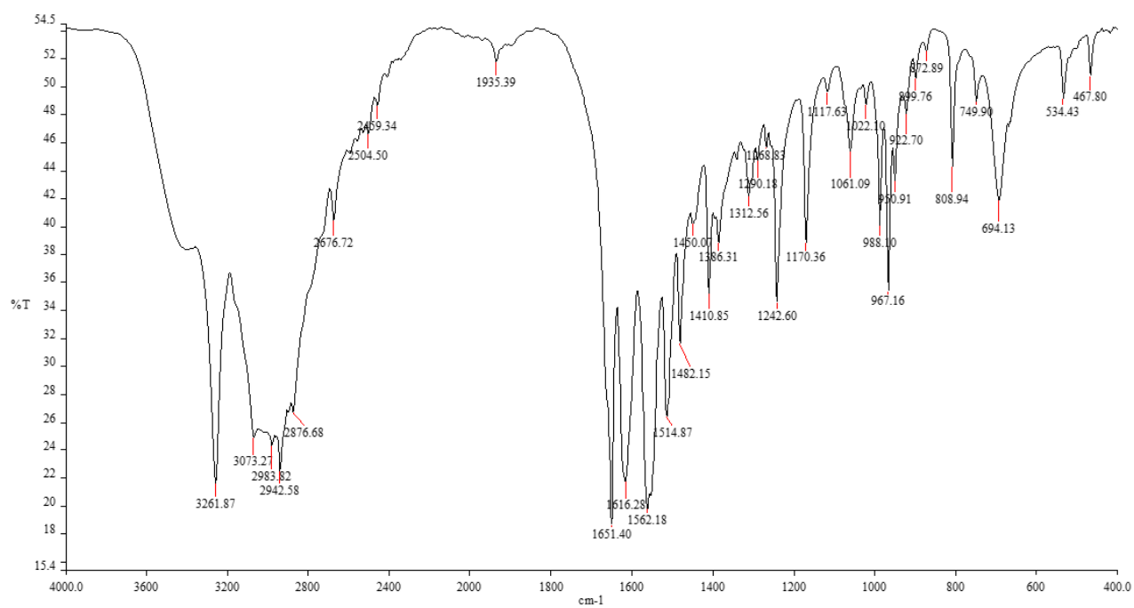
Figure S24. FTIR spectrum (KBr) of compound 11b.
