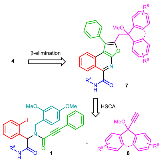
Scheme 3 Retrosynthetic plan.
